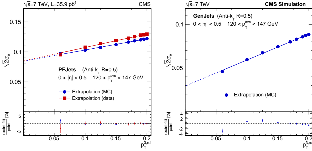
Figure 30. Examples of extrapolations of \sqrt{2}\sigma_{rel} as a function of p_T^{Jet3}/p_T^{ave} to zero for PF jets ( R = 0.5 ) in |\eta| < 0.5 and 120 < p_T^{ave} < 147 GeV (left). Example of a corresponding extrapolation for MC particle jets (right).
