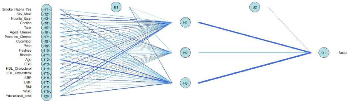
Fig. 4.3 Neural Network Architecture. Input units: from I1 to I20; Hidden units: from H1 to H3; Output unit: O1. B1 and B2 are, respectively, hidden neuron bias and output neuron bias.
