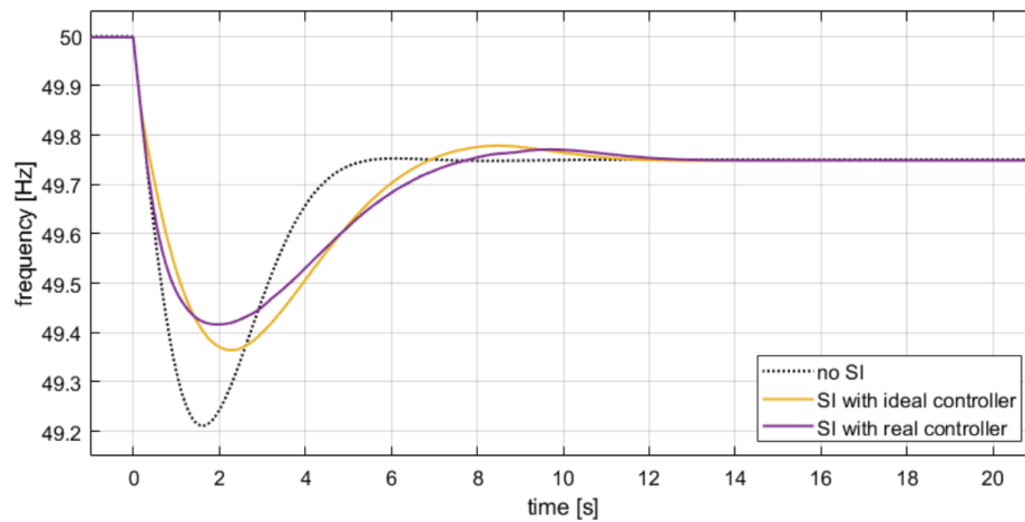
Figure 3.26: System frequency behavior with SI contribution by low-cost controller
