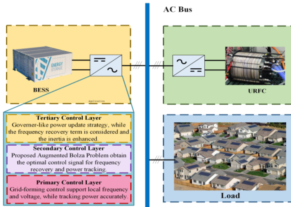
Figure 3.19: Architecture of the microgrid model under study
