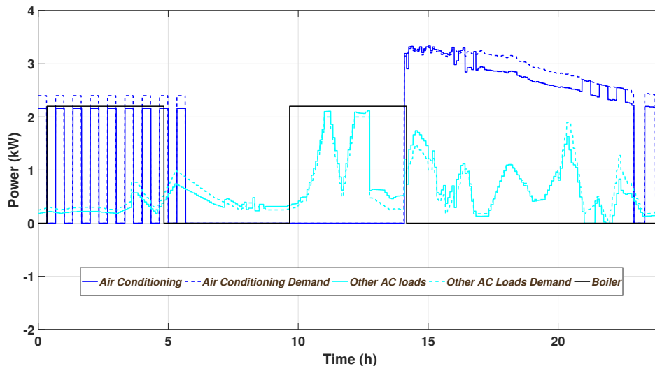
Figure 2.2: AC loads profiles
