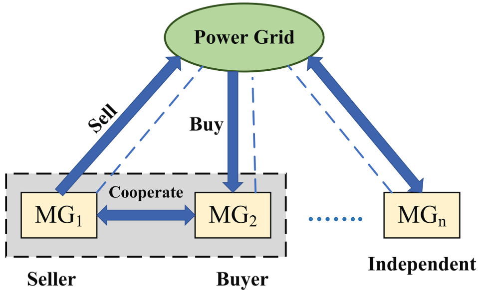
Figure 2.6: Transactive energy framework of MMGs
