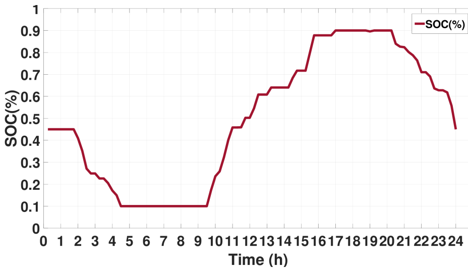
Figure 2.19: BESS SOC (%)
