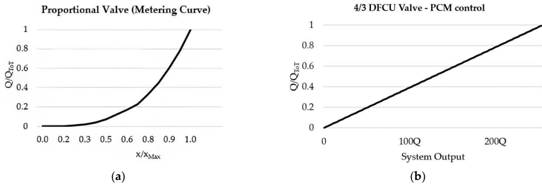
Fig. 47. Comparison between analogue and digital hydraulic valves: (a) Proportional Valve; (b) 4/3 DFCU Valve, adapted from [117].
