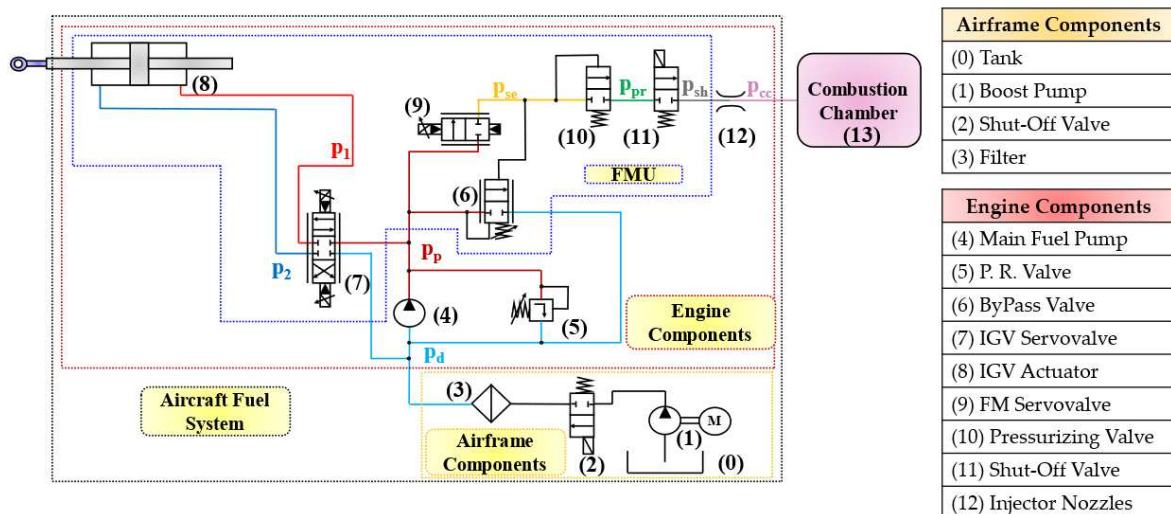
Fig. 77. Aircraft fuel system layout analysed in this research project.
