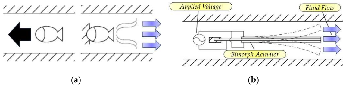
Fig. 71. Bionic bimorph valveless piezopump: (a) Fish propulsion; (b) Pump scheme.
