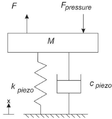
Fig. 126. Piston and piezostack force diagram.
