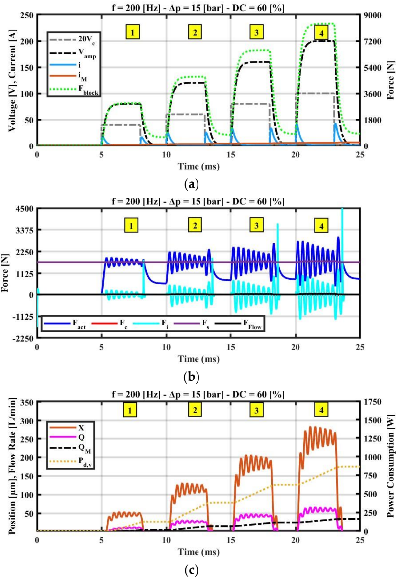
Fig. 101. Open-loop predictions simulated for different values of V_c ( f = 200 Hz, \Delta p = 15 bar, DC = 60\% ): (a) Amplitude of the Input Control Voltage, Amplified Voltage, Current, Average Current, Blocking Force; (b) Actuation Force, Viscous Force, Inertia Force, Additional Spring Force, Flow Force; (c) Poppets' Position, Flow Rate, Average Flow Rate, Ideal Average Power Dissipated by the Valve.
