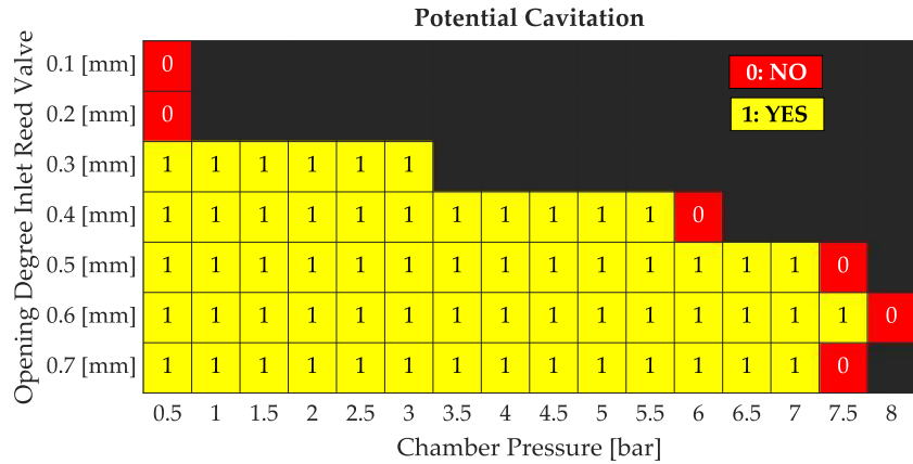
Fig. 160. Possible cavitation scenarios considering p_{in} = 20 bar and varying v_{opn} from 0.1 mm to 0.7 mm (increments of 0.1 mm) and p_{cham} (increment of 0.5 bar starting from 0.5 bar).
