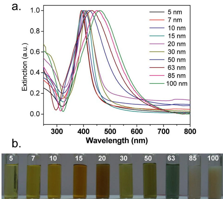
Fig. 1.5 : In a) UV-Vis extinction spectra and (b) the distinctive colour of different sized Ag NPs. [52]
