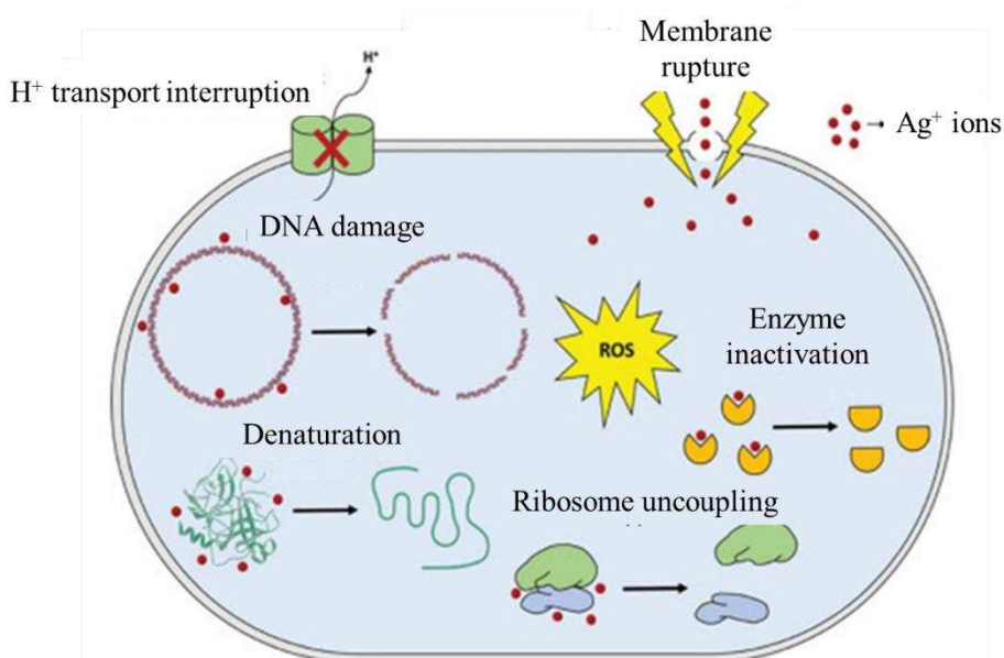
Fig. 1.7: Schematic illustration of the antibacterial mechanism of Ag nanostructures. [54]
