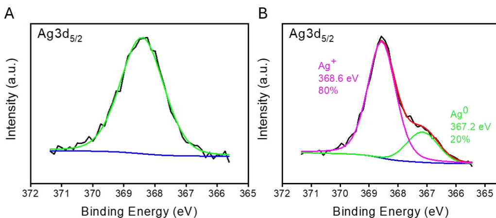
Fig.4.7: \text{Ag}3d_{5/2} high resolution XPS spectra of A) Cot/AgNPs and B) Cot/His-RGO/AgNPs samples aged for 60 days.
