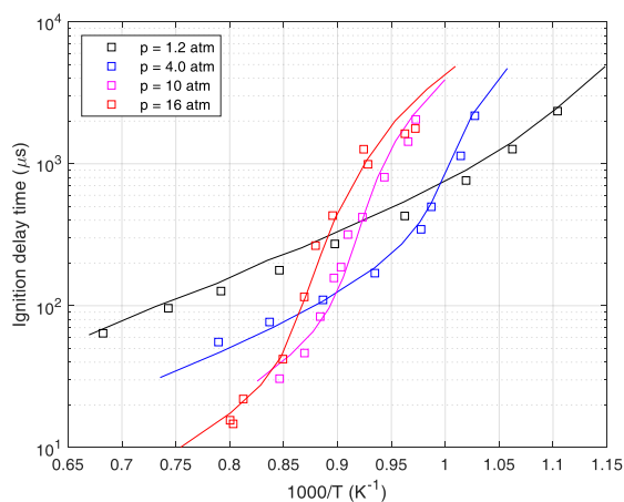
Figure 2-2 Performance of Kéromnès kinetic mechanism [57] against shock tube experiments [54] at \phi = 1 and pressures equal to 1.2, 4.0, 10 and 16 atm. Square markers represent experimental data and solid lines represent numerical simulations.
