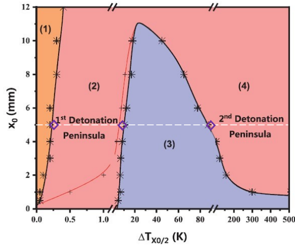
Figure 5-7 Detonation response diagram for H 2 /air at T_0 = 1050 \text{ K} and p_0 = 40 \text{ atm} in planar coordinates (adapted from [140]). Simulation results from present work (purple diamond markers) using detonationFoam solver [159] have been superimposed for comparison.
