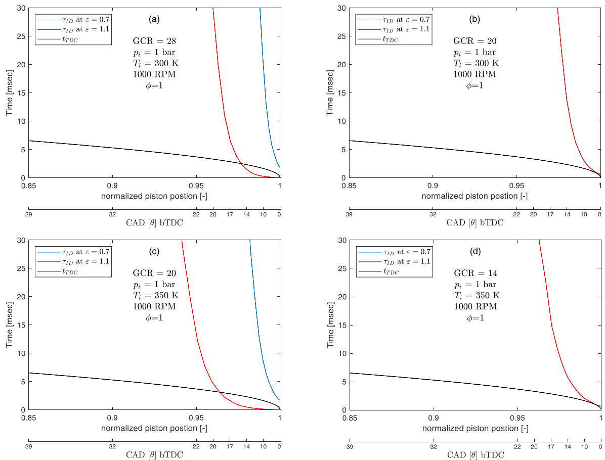
Figure 3-8 Transition from unsafe to safe conditions by varying GCR and intake temperature. (a) Arbitrary unsafe condition where \tau_{ID} gets lower than t_{TDC} in the TDC vicinity for \varepsilon = 1.1 . (b) Marginally safe condition satisfying the tangency criterion by reduction in GCR from 28 to 20. (c) Reinstating an unsafe condition by increasing the intake temperature T_i to 350\text{ K} . (d) Obtaining a safe condition again by further reduction in GCR to 14 while keeping T_i = 350\text{ K} .
