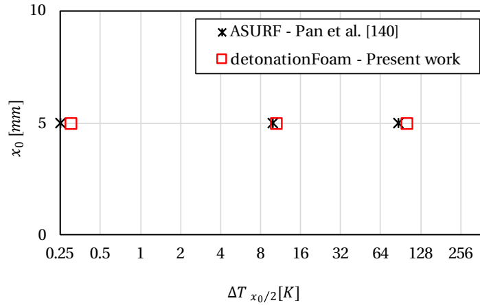
Figure 5-6 Validation of solver ‘detonationFoam’ against literature data [140] at x_0 = 5 \text{ mm} with linear temperature gradient inside hot spot.
