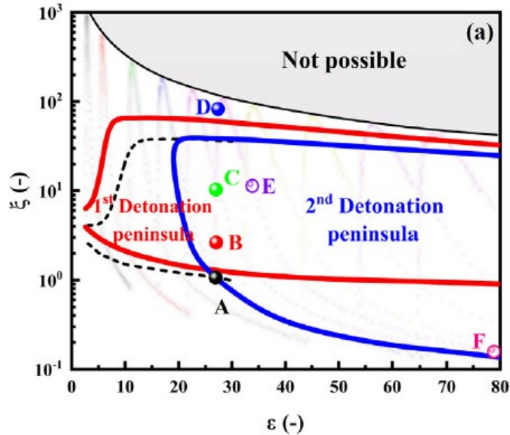
Figure 5-1 Detonation diagram in spherical coordinates. \xi - \epsilon diagram. The dashed lines denote the results of Ref. [130]. Figure adapted from [139].
