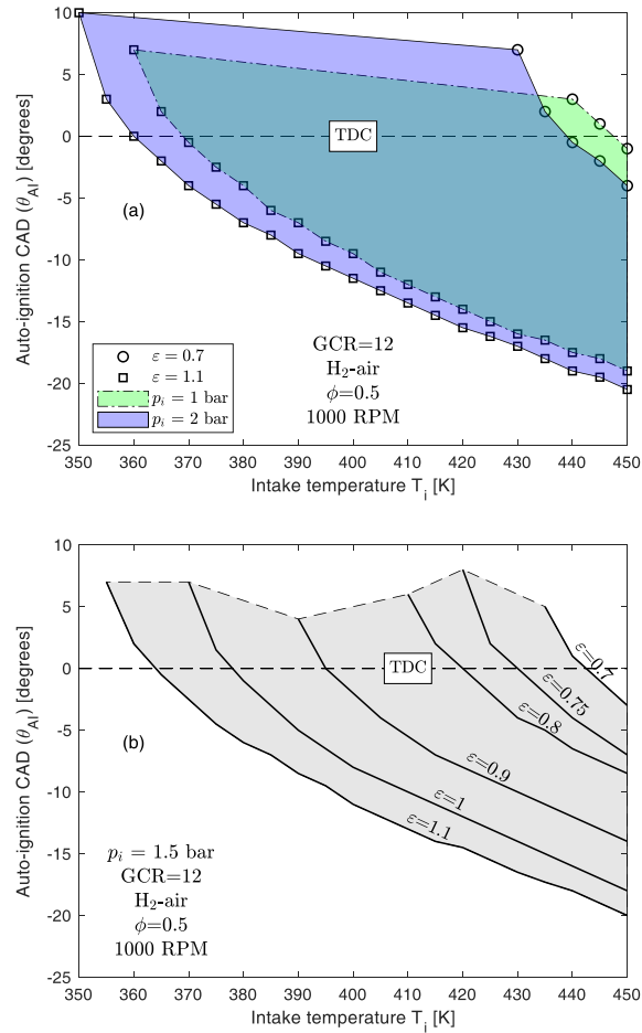
Figure 3-12 Auto-ignition CAD \theta_{AI} across a range of intake temperatures for (a) p_i = 1 bar and p_i = 2 bar (b) p_i = 1.5 bar with iso- \epsilon lines.
