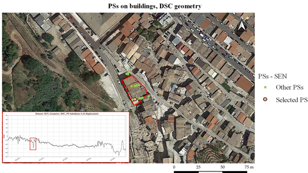
Fig. 63 - Identification of the structures object of subsidence (red polygon), distribution of PSs, and time-displacement series of on PS.
