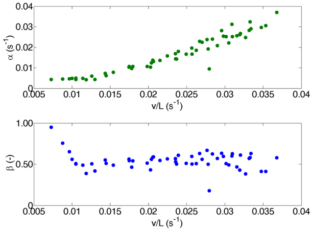
Figure 7. Mass transfer coefficient \alpha and fraction of mobile water \beta as function of normalized velocity v/L ( \text{s}^{-1} ) for MIM. An outlier is evidenced for v/L = 0.028 \text{ s}^{-1} .
