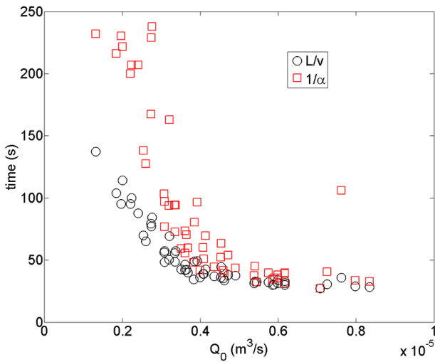
Figure 8. Transport time ( L/v ) (reciprocal of normalized velocity) and exchange time ( 1/\alpha ) (reciprocal of the exchange term) as function of injection flow rate Q_0 ( \text{m}^3 \text{ s}^{-1} ) for MIM.
