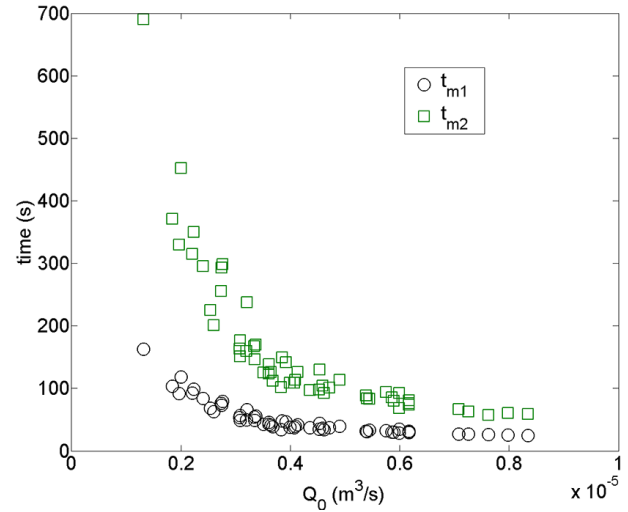
Figure 9. Travel time for main path t_{m1} (s) and travel time for secondary path t_{m2} (s) for ENM4 as function of injection flow rate Q_0 ( \text{m}^3 \text{ s}^{-1} ).
