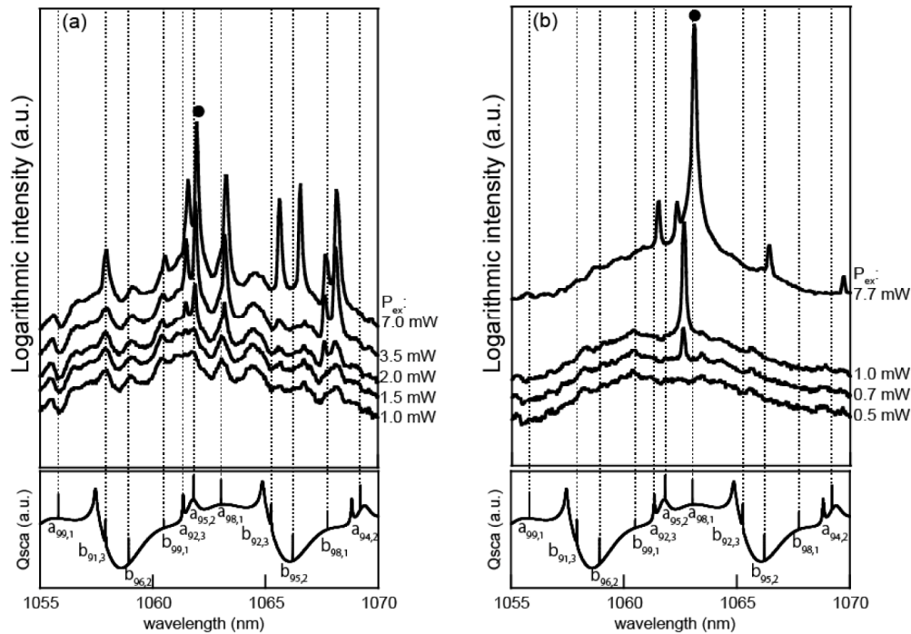
Fig. 3. Emission spectra from (a) uncoated and (b) terrace microspheres at various excitation powers. Pumping positions for (a) and (b) were the edge of the sphere and that of the terrace, respectively, and the pumping wavelengths were 803.5 and 805.3 nm, respectively. The power of the CW Ti:sapphire laser irradiated on each sample is represented by P_{\text{ex}} . The bottom spectra are based on Q_{\text{sca}} values calculated using Mie theory for a 28.82- \mu\text{m} microsphere. The dotted lines indicate the resonance wavelengths of WGMs. The parameters a_{n,l} and b_{n,l} are the transverse magnetic and electric modes, respectively. The subscripts n and l indicate the mode number and order of each resonance, respectively.
