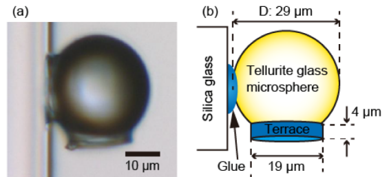
Fig. 2. (a) Optical photograph of a terrace microsphere attached to a silica glass substrate. (b) Schematic of the terrace microsphere.
