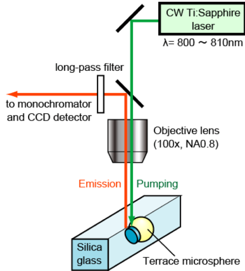
Fig. 1. Schematic of the experimental apparatus used to pump the terrace microsphere and obtain its emission spectrum.
