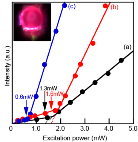
Fig. 4. Plots of emission intensities of (a) uncoated and (b, c) terrace microspheres versus the excitation power of the Ti:sapphire laser. Pumping positions are the edge of the sphere, center of the terrace, and edge of the terrace for (a), (b), and (c), respectively. Solid lines indicate the least-squares fitting results, and the lasing threshold is given by the intersection of curves with the horizontal axis. The inset photograph is the terrace microsphere pumped above the laser threshold.
