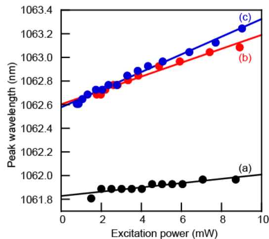
Fig. 5. Peak wavelengths versus excitation power for (a) uncoated and (b, c) terrace microspheres. Solid lines represent the least-squares fitting results. Pumping positions were the (a) edge of the sphere, (b) center of the terrace, and (c) edge of the terrace.
