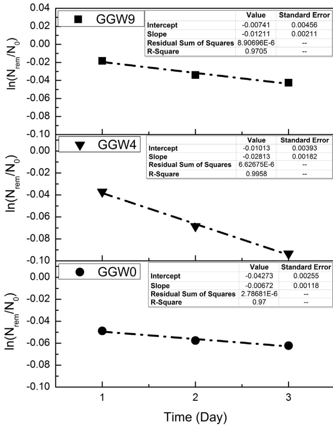
Fig. 2. The values for the nitrogen release rate constant ( k , – slope of plot), their related correlation ( R^2 ), and \beta values ( y -intercept) obtained for the three days of rain simulations applied on each of the three compost ages GGW0, GGW4 and GGW9 for the inter-storm model.
