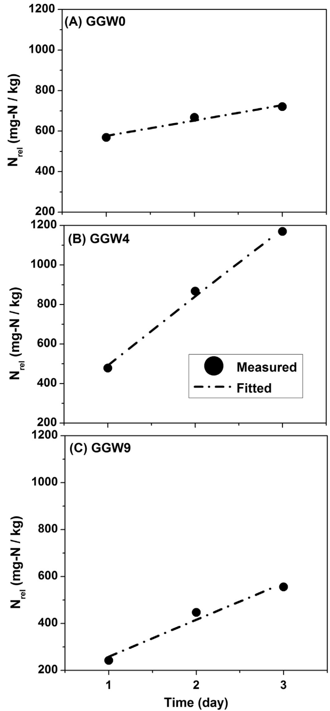
Fig. 3. Measured (data points) and predicted (dashed line) values of total nitrogen release for the three compost types on the three consecutive simulated storm events. Inter-storm results for GGW0, GGW4 and GGW9 are presented in sub-figures A, B, and C, respectively.
