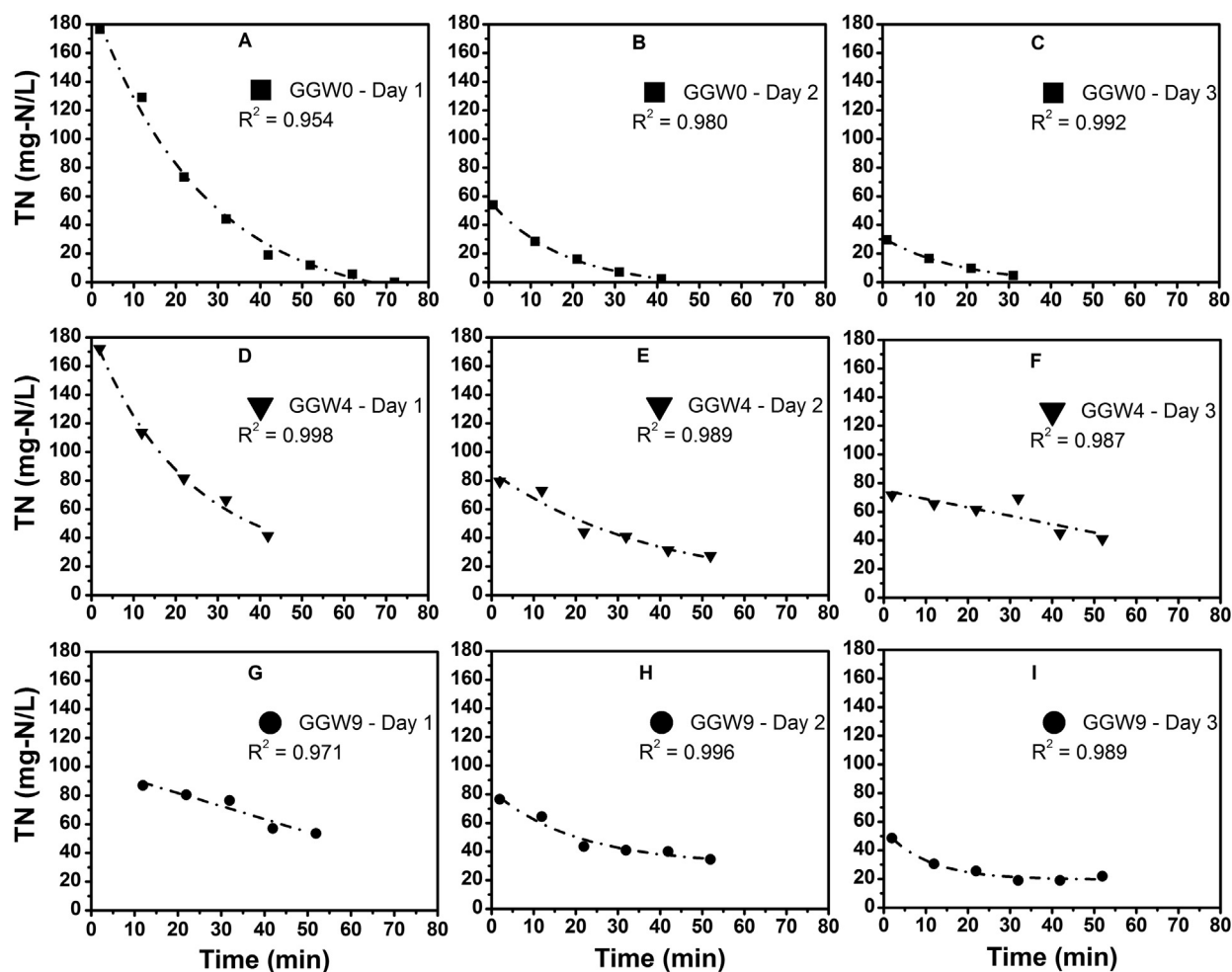
Fig. 1. Measured (data points) and predicted (dashed line) values for total nitrogen concentration in runoff for the three compost types during the three consecutive simulated storm events. Results for GGW0 for storm days 1, 2, and 3 are presented in sub-figures A, B, and C respectively. Similarly for GGW4 storm days 1, 2, and 3 are presented in sub-figures D, E, F, and for GGW9 storm days 1, 2, and 3 are presented in sub-figures G, H, and I.
