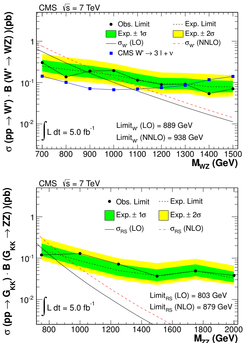
Figure 4. Observed and expected 95% CL upper cross section limits and comparison with the theoretical predictions in W' (top) and RS graviton with k/\overline{M}_{Pl} = 0.05 (bottom) models for the combination of electron, muon, and E_T^{\text{miss}} channels. The limits are calculated with the modified frequentist CL_s statistical method.
