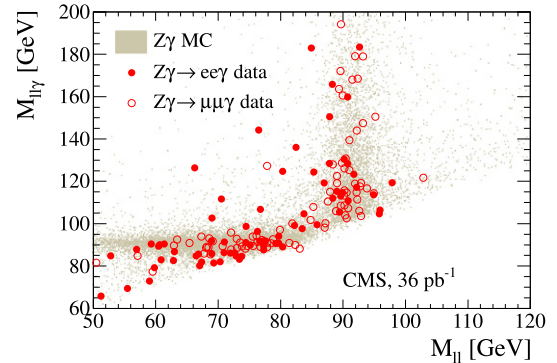
Fig. 5. Distribution of the \ell\ell\gamma invariant mass as a function of the dilepton invariant mass for selected Z\gamma candidates in the electron (filled circles) and muon (open circles) final states. The data accumulation at M_{\ell\ell\gamma} \simeq M_Z corresponds to FSR events, while the data at M_{\ell\ell} \simeq M_Z correspond to ISR events.
