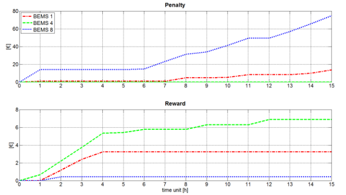
Figure 5. Cumulative reward and penalty profiles of buildings b_1 , b_4 and b_8 .
