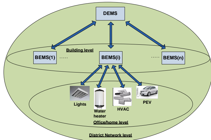
Figure 1. The district energy management architecture.
