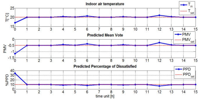
Figure 6. T_{in} , PMV and PPD of b_1 obtained by the optimization.
