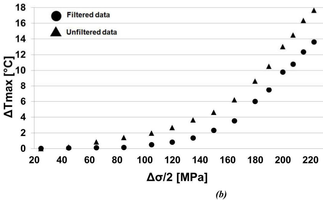
Figure 5 (a). Filtered and unfiltered temperature data, specimen 1, ASTM A 182 grade F6NM, (b). Filtered and unfiltered temperature data, specimen 1 X4 Cr Ni Mo 16-5-1.
