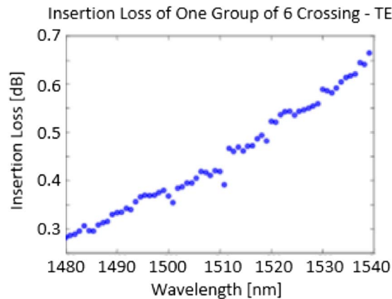
Fig. 15. Insertion loss of one group of six crossings for TE polarization.
