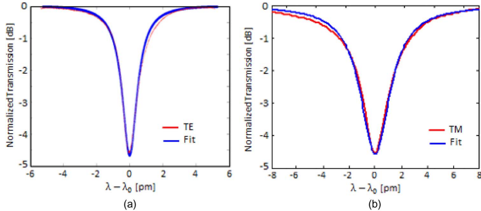
Fig. 17. Ring resonator spectrum for the TE (a) and the TM (b) polarization. Lineplots represent the fit to the theoretical equations.
