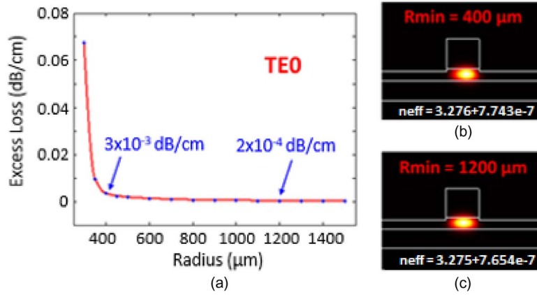
Fig. 3. Excess loss vs. radius for TE 0 mode (a). Modal distribution related to TE 0 in the shallow waveguide with a bending radius of 400 \mu\text{m} (b) and 1200 \mu\text{m} (c).
