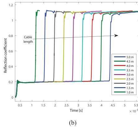
Fig. 5. Measured reflectograms for cable lengths from (a) 10 to 50 cm and (b) 1 to 5 m.
