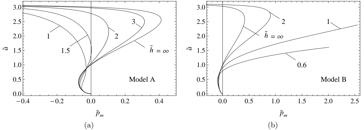
FIG. 7: The dimensionless contact size \tilde{a} at the equilibrium as a function of the dimensionless mean contact pressure \tilde{p}_m for different values of the dimensionless layer thickness \tilde{h} , \tilde{\Lambda} = 2 and \tilde{\gamma} = 0.05 . Results are shown both for the model A (a) and the model B (b).
