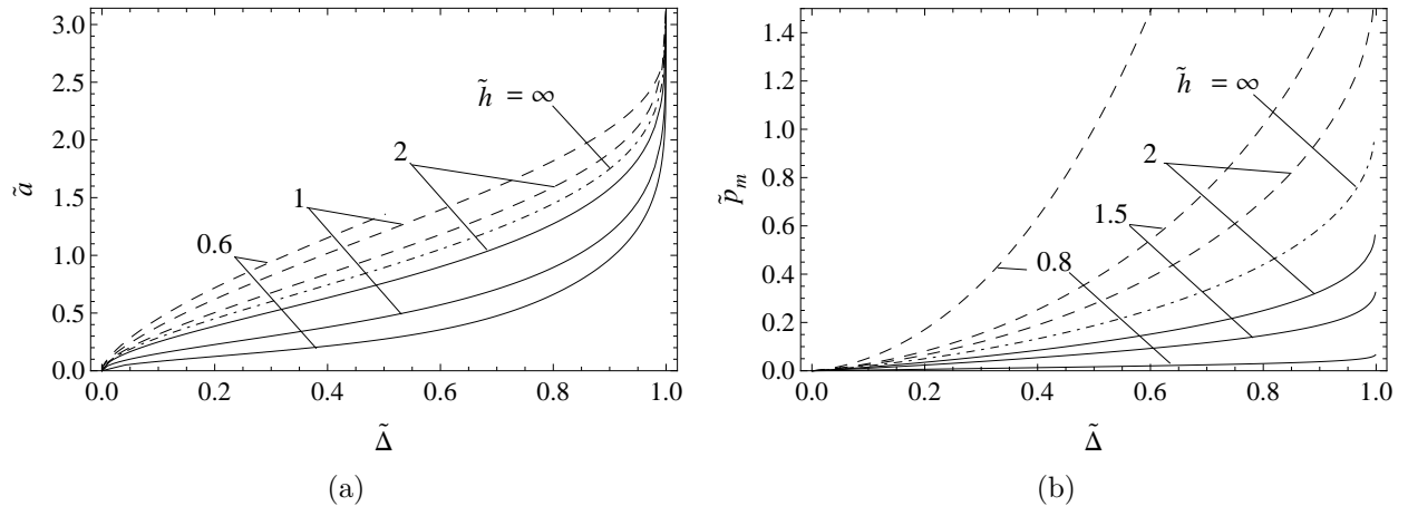
FIG. 10: The dimensionless contact size \tilde{a} (a) and mean pressure \tilde{p}_m (b) at the equilibrium as functions of the dimensionless contact penetration \tilde{\Delta} , for different values of the dimensionless layer thickness \tilde{h} . Solid lines refers to the model A, dashed lines to the model B. The halfplane solution [51] is plotted with dashed-dot line.
