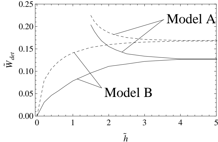
FIG. 9: The dimensionless energy dissipated during the pulling process as a function of the layer thickness. Calculations are performed under force controlled (solid lines) and displacement controlled (dashed lines) conditions. The displacement corresponding to the equilibrium state with positive contact area and no applied external load has been used as initial condition. Results are given for \tilde{\Lambda} = 2 and \tilde{\gamma} = 0.05 .
