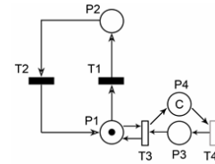
Fig. 4b. Railway subnet model: incoming and outgoing ITUs.
