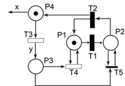
Fig. 4c. Railway subnet model: incoming and outgoing ITUs with separate load/unload.
