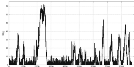
Fig. 16. M(P_{27}) (occupation of access road) in Scenario 3.
