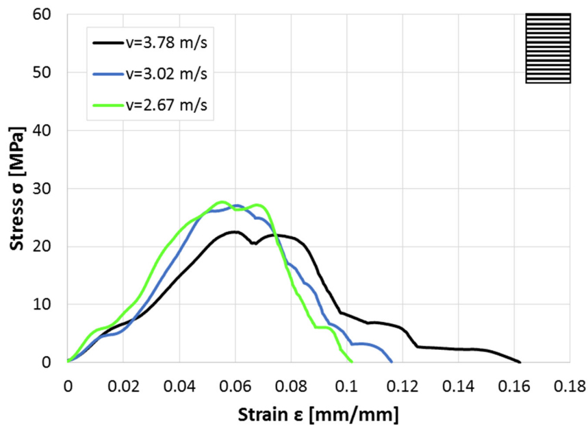
Figure 8.22 Single-layer stress-strain curve for 90° specimen and for each impact speeds
