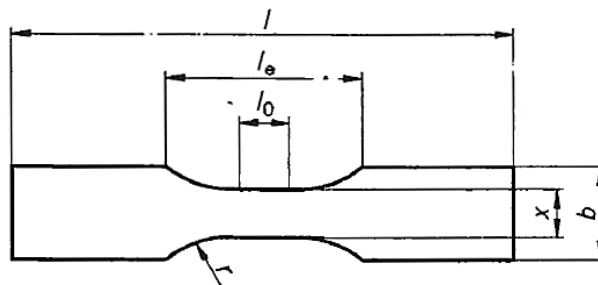
Figure 8.9 Type III specimen shape
