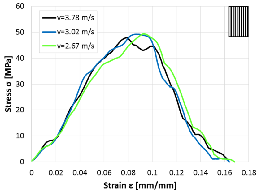
Figure 8.20 Single-layer stress-strain curve for 0° specimen and for each impact speeds
