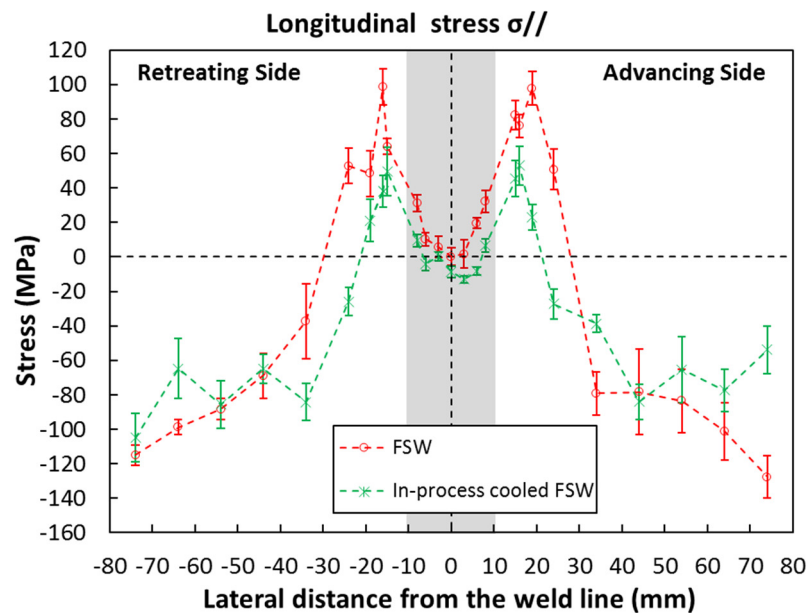
Figure 5.5 Comparison between longitudinal residual stresses in FSW and in-process cooled FSW
