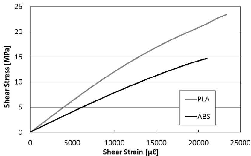
Figure 8.6 Representative shear stress - shear strain data for both PLA and ABS
