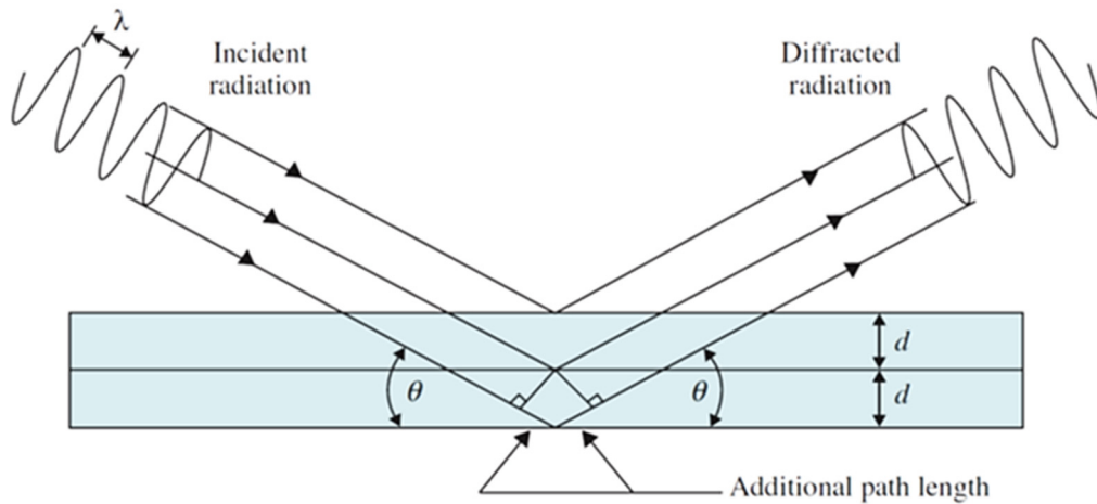
Figure 2.9 Radiation diffraction within a crystal structure [5]
