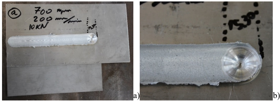
Figure 5.9 Lap joint aluminium-titanium (a) and a detail of the welded bead (b)
