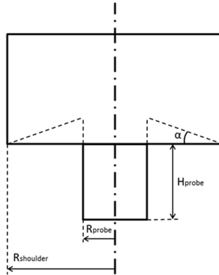
Figure 4.7 Tool scheme
