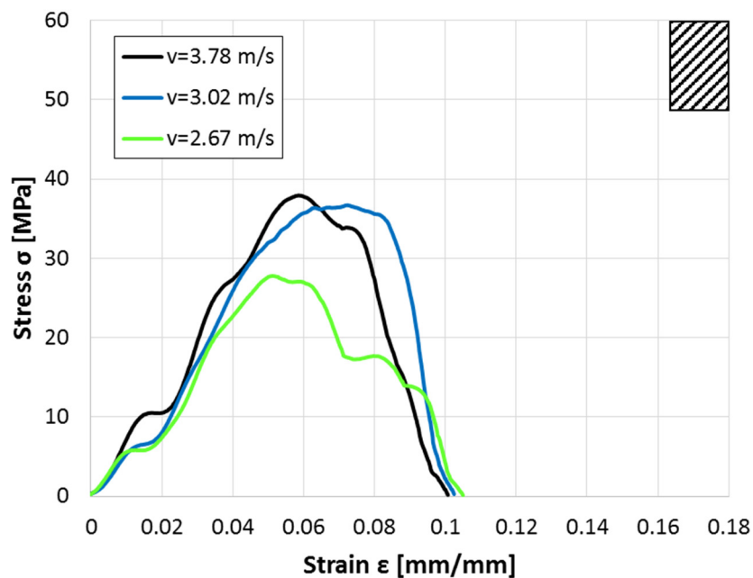
Figure 8.21 Single-layer stress-strain curve for 45° specimen and for each impact speeds
