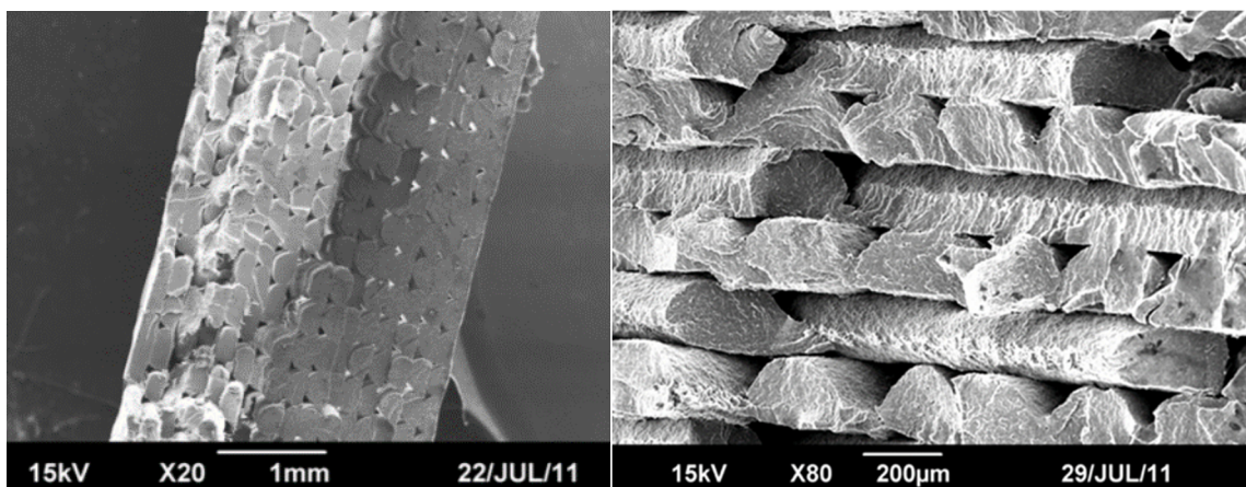
Figure 7.2 FDM fracture section through a SEM image [69]
