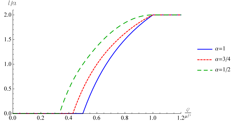
Figure 3.5. Dimensionless slip distance l/a as a function of \frac{Q}{fP} for different values of \alpha = [1 - 3/4 - 1/2] .
