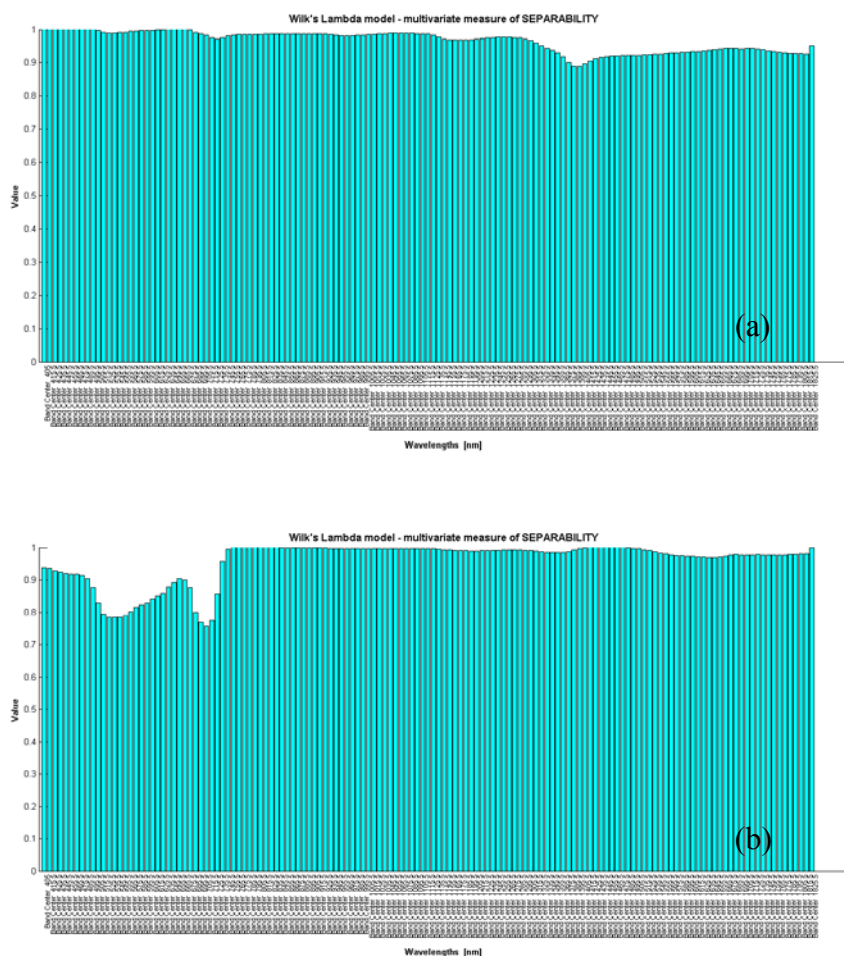
Fig. 3/11 - Spectrum of separable potentials between healthy and infected leaves of both varieties: (a) Celina di Nardò and (b) Leccino.
