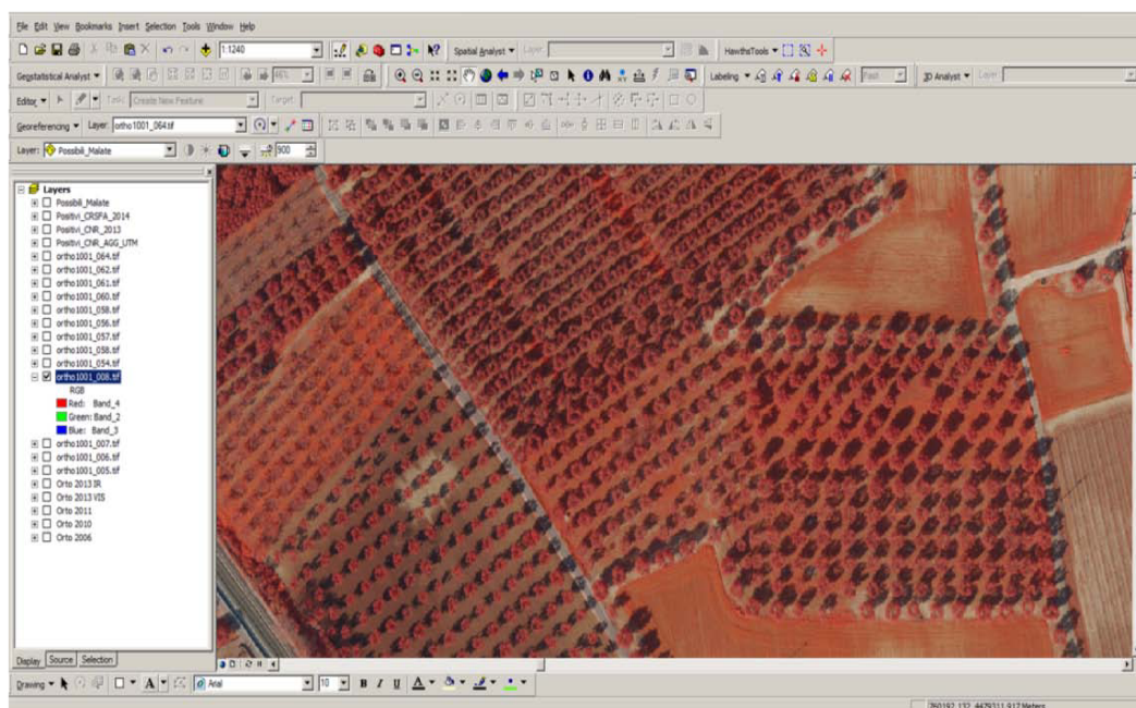
Fig. 2/3 - Images in false color, used in the photointerpretation phase manual, within the GIS framework.
