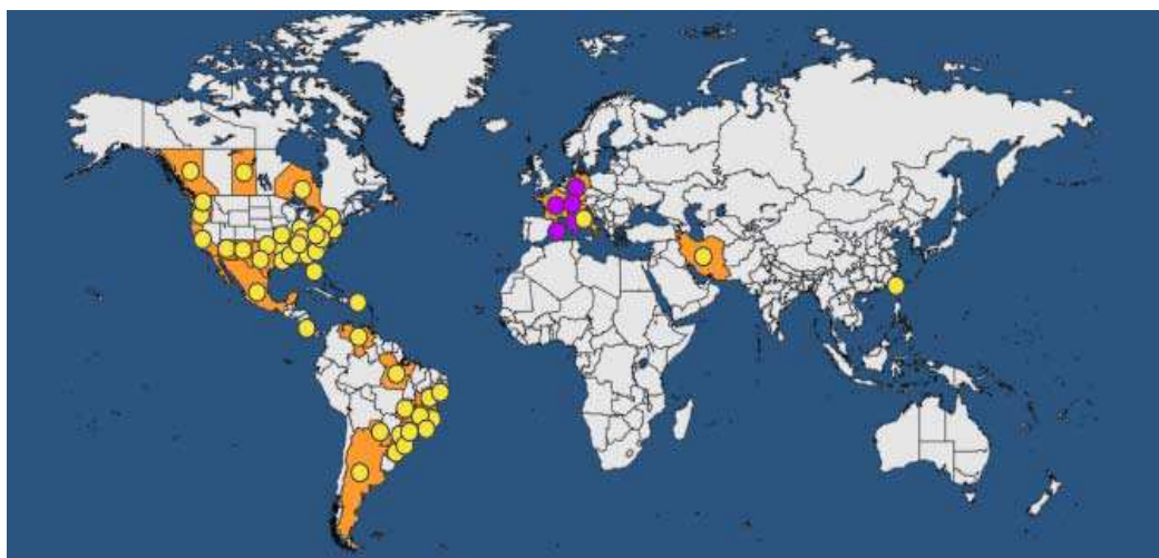
Fig. 1/2 - World distribution of Xylella fastidiosa (EPPO, 2016).
