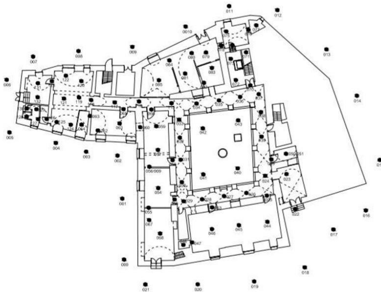
Fig. 22 Acquisition plan where coded dots represent scan position (Santa Croce Monastery, Modugno, Italy)
