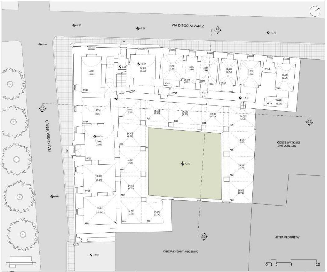
Fig. 85 Ground floor plan
