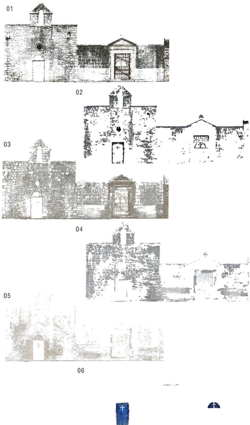
Fig. 55 Clusters in HSV (Case 3-façade Est): 1) biological colonization (46%); 2) spots/deposit (17%);3) moist area (75%); 4) biological patina (67%) 5) unaltered surface (24%);6) doors (7%)
