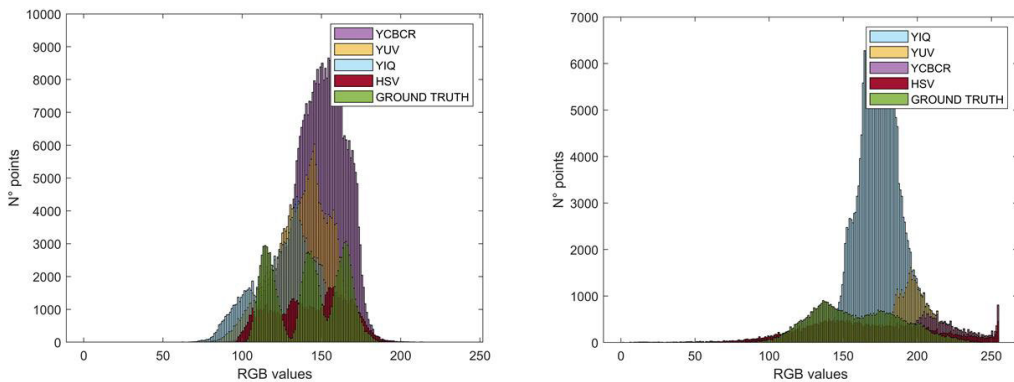
Fig. 59 Overlapping between analogous clusters histograms (unified RGB) of the four colour spaces and the ground truth. Case 2: moist area (left); staining (right)(Musicco et al., 2021).
