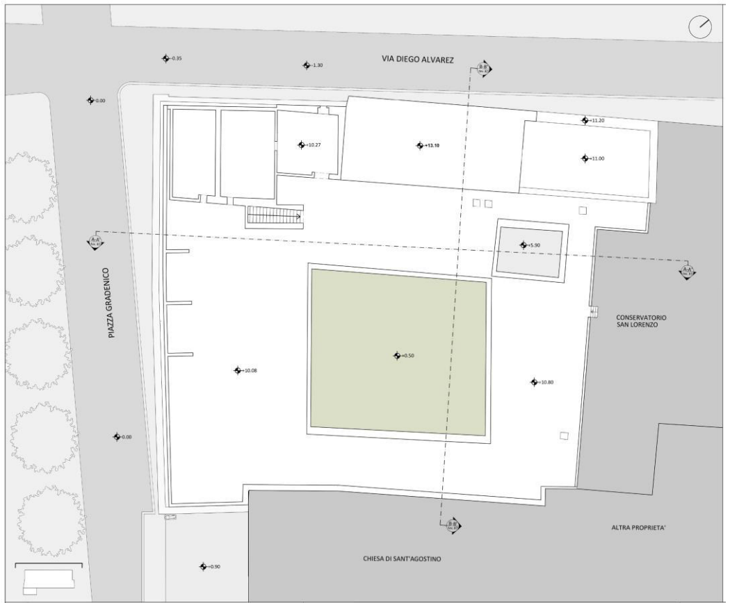
Fig. 87 Roofing plant
