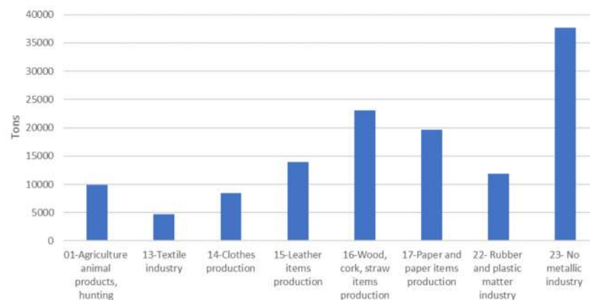
Figure 7. Non-hazardous waste production (tons) in Puglia considering different activities—2019 (Adapted from ISPRA [32]).
