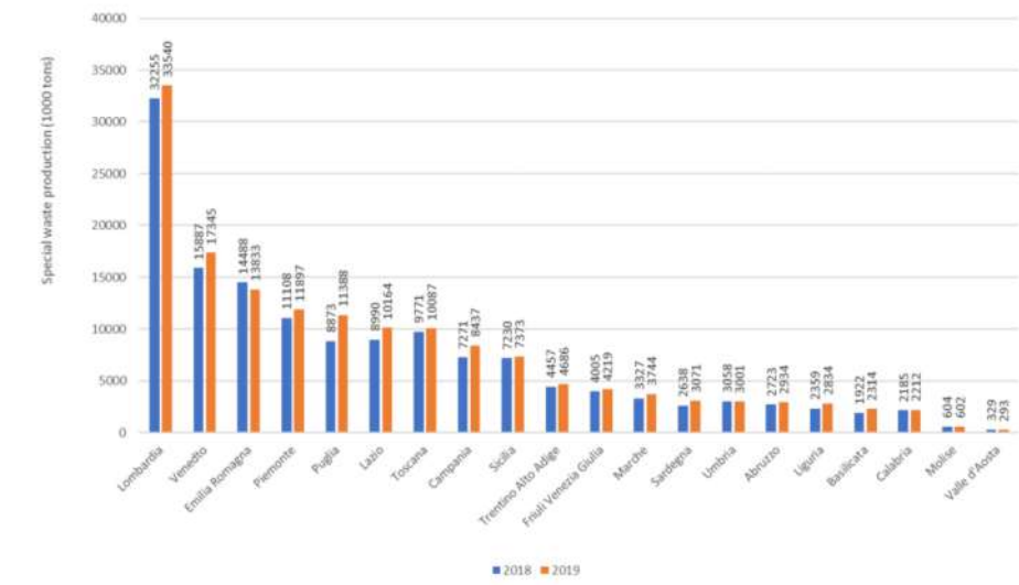
Figure 6. Total production of special waste at regional level from 2018 to 2019 (Source: Rapporto rifiuti speciali, ISPRA [35]).
