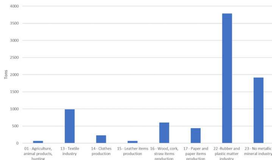
Figure 8. Non-hazardous waste production (tons) in Molise region considering different activities—2019 (Adapted from ISPRA [32]).
