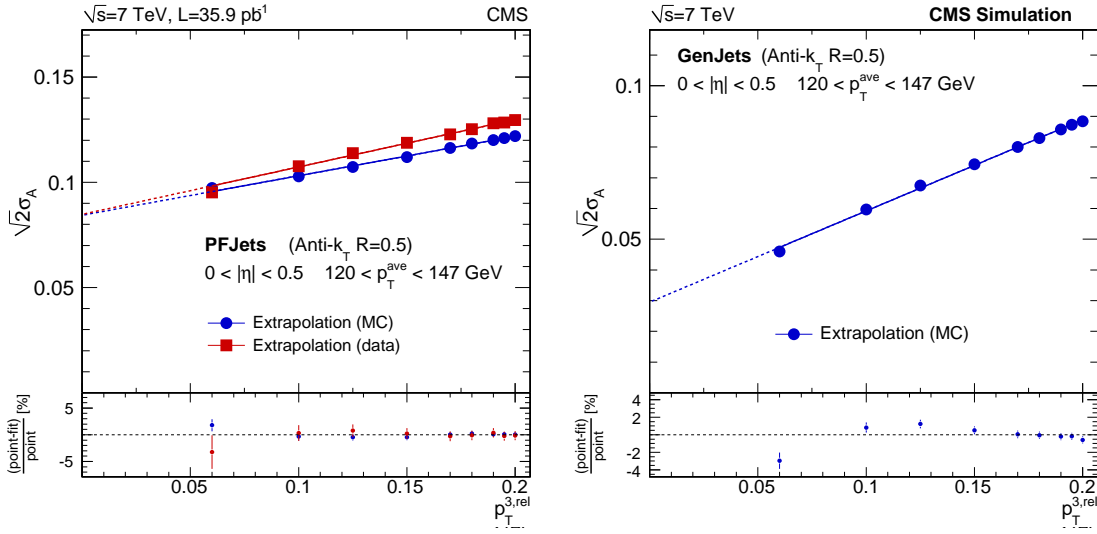
Figure 30. Examples of extrapolations of \sqrt{2}\sigma_d as a function of p_T^{\text{Jet}3}/p_T^{\text{ave}} to zero for PF jets ( R = 0.5 ) in |\eta| < 0.5 and 120 < p_T^{\text{ave}} < 147 \text{ GeV} (left). Example of a corresponding extrapolation for MC particle jets (right).
