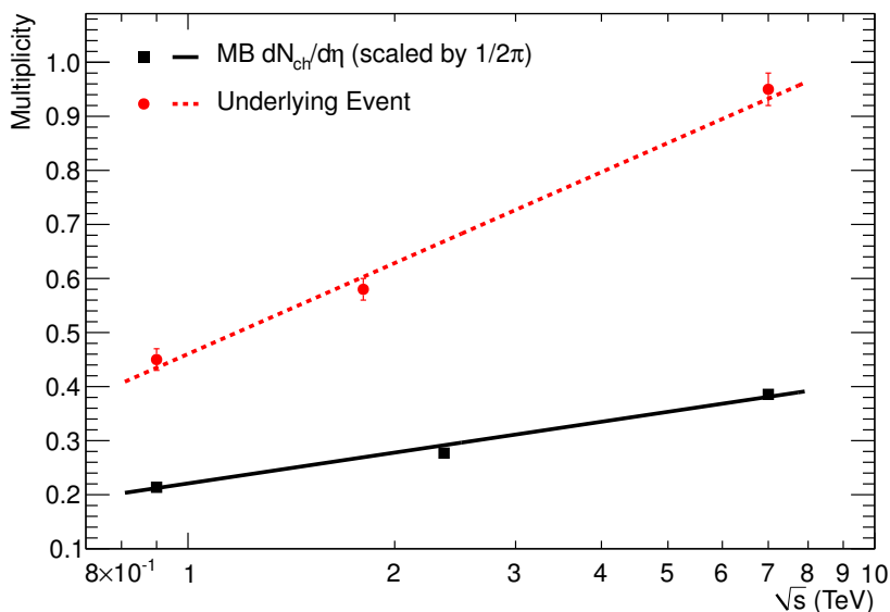
Figure 7. Comparison of number density in the plateau of the Transverse region (see table 8) and dN_{\text{ch}}/d\eta in minimum-bias events (scaled by 1/2\pi ) [32]. Both are for charged particles with p_T > 0.5 \text{ GeV}/c . For this plot, statistical and systematic uncertainties have been summed in quadrature. The lines show fits with the functional form a + b \ln s .
