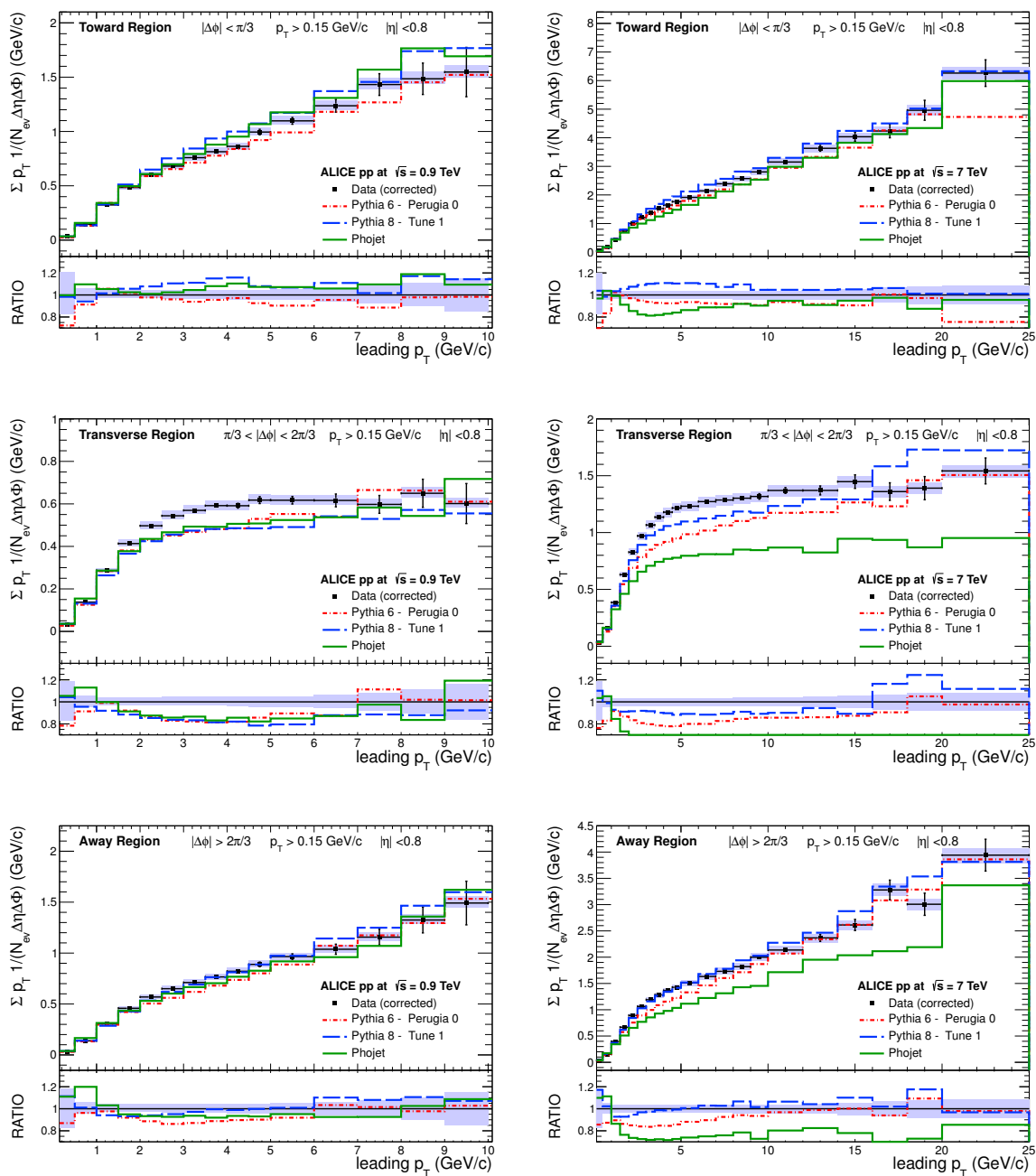
Figure 9. Summed p_T in Toward (top), Transverse (middle) and Away (bottom) regions at \sqrt{s} = 0.9 \text{ TeV} (left) and \sqrt{s} = 7 \text{ TeV} (right). Right and left vertical scales differ by a factor 4 (2) in the top (middle and bottom) panel. Shaded area in upper plots: systematic uncertainties. Shaded areas in bottom plots: sum in quadrature of statistical and systematic uncertainties. Horizontal error bars: bin width.
