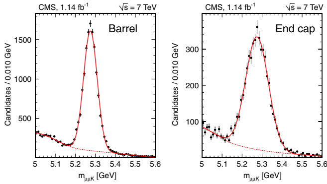
FIG. 3 (color online). B^+ \rightarrow J/\psi K^+ invariant mass distributions in the barrel (left) and end cap (right) channels. The solid (dashed) lines show the fits to the data (background).
