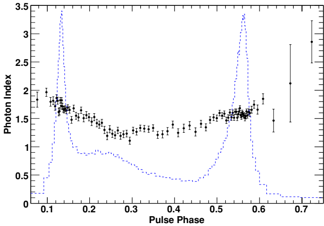
Figure 8. Photon index vs. phase from fits in fixed-count phase bins of 1500 photon counts per bin. The error bars denote statistical errors. (A color version of this figure is available in the online journal.)
