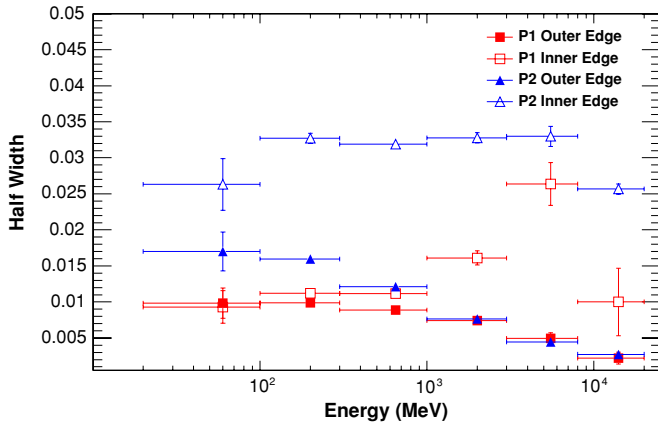
Figure 3. Measured HWHM of P1 and P2 from two-sided Lorentzian fits as a function of energy.
