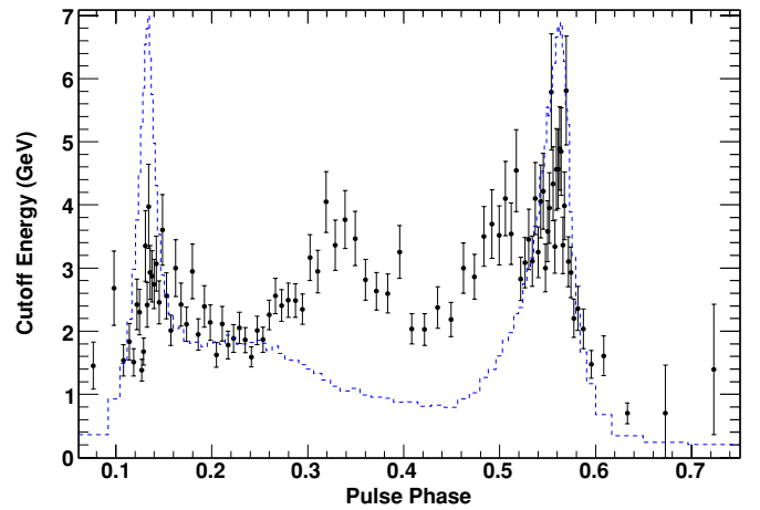
Figure 9. Spectral cutoff energy vs. phase from fits in fixed-count phase bins of 1500 photon counts per bin. The solid error bars denote statistical errors. (A color version of this figure is available in the online journal.)
