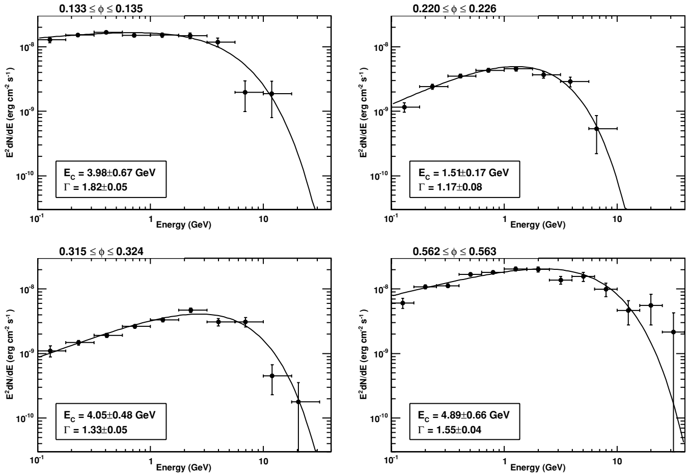
Figure 10. Spectral energy distribution in four phase intervals of Figure 9. The individual spectra have been exposure corrected to account for the fact that the fitting was done in a small phase bin.
