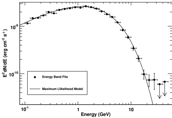
Figure 7. Phase-averaged spectrum for E > 0.1 –100 GeV.
