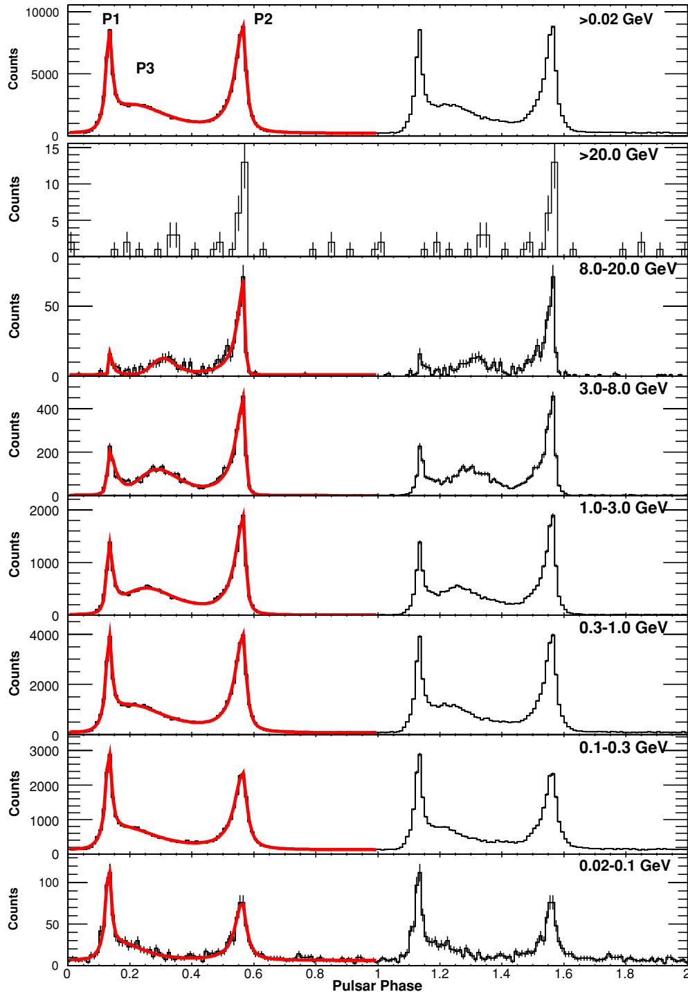
Figure 2. Light curves for different energy bands over two pulse periods. Joints fits of P1, P2, and P3 in each energy band (as described in the text) are superposed on the light curves in the first cycle.
