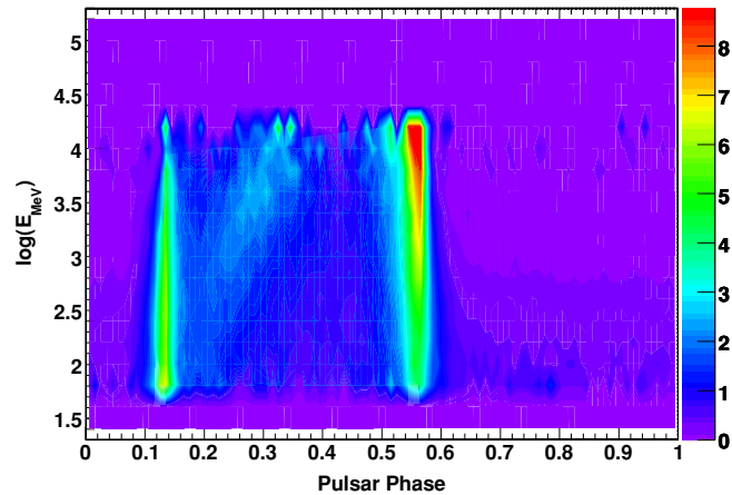
Figure 5. Plot of pulse profile as a function of energy. The color scale is relative counts in each bin on a linear scale.
