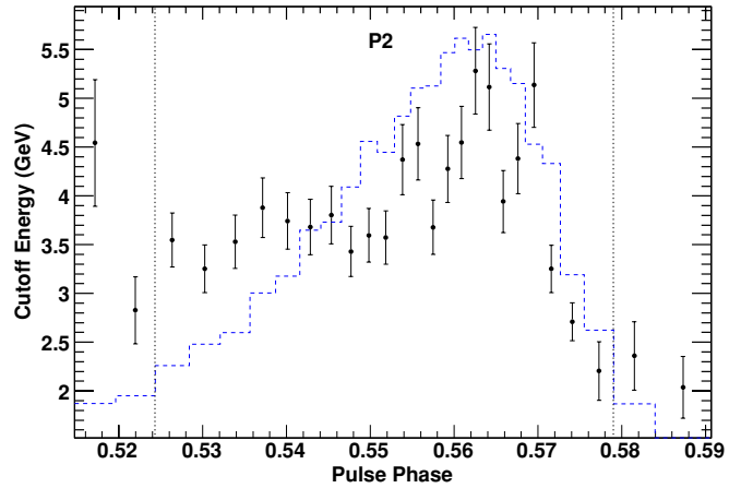
Figure 12. Spectral cutoff energy vs. phase in P2 from fits in fixed-count phase bins of 1500 photon counts per bin, where the photon index was held fixed to a value of 1.58 \pm 0.01 over the phase range between the dotted lines.
