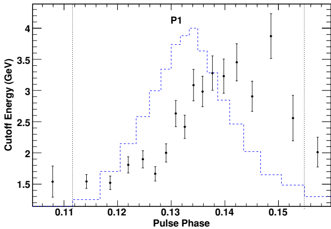
Figure 11. Spectral cutoff energy vs. phase in P1 from fits in fixed-count phase bins of 1500 photon counts per bin, where the photon index was held fixed to a value of 1.72 \pm 0.01 over the phase range between the dotted lines.
