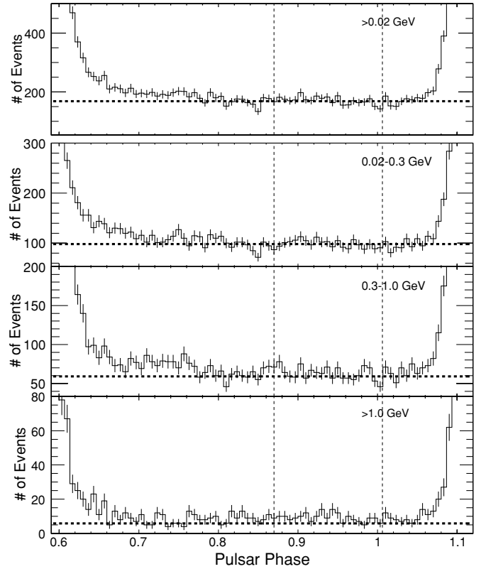
Figure 6. Detail of the off-pulse phase region for 150 equal-size phase bins for the full energy range 0.02–300 GeV and in three different energy bands. The horizontal dashed line denotes the background level determined from a simulation (see Section 3.2.2). The dashed vertical lines mark the phases of the RXTE P3 and P4 (Harding et al. 2002).
