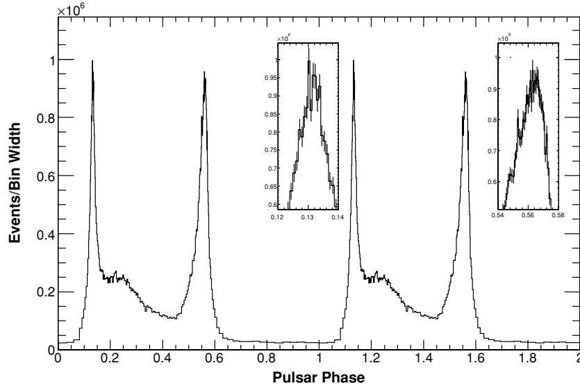
Figure 1. Light curve for energy range 0.02–300 GeV for 203 fixed-count phase bins with 750 photons per bin. Insets show details of P1 and P2.
