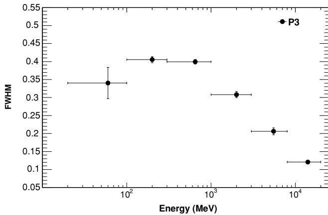
Figure 4. Measured width (FWHM) of P3 as a function of energy.
