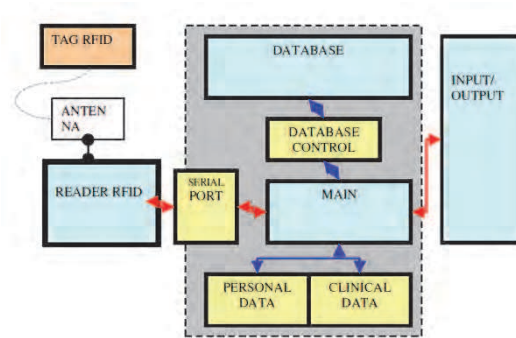
Fig. 23. Block diagram of the hardware part of the designed RFID-based system
