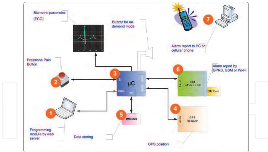
Fig. 17. Pain Button (PB) block diagram
