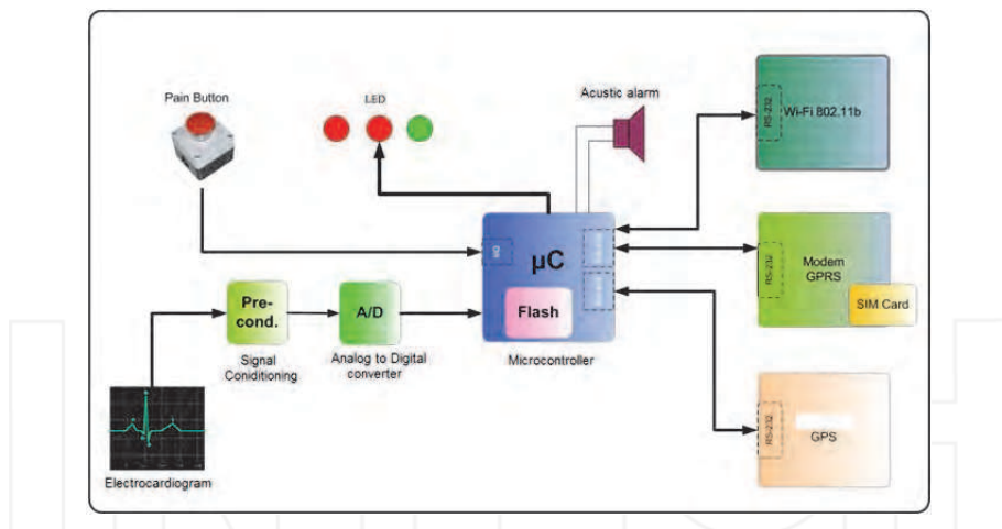
Fig. 18. Wireless Pain Button (WiPB) block diagram
