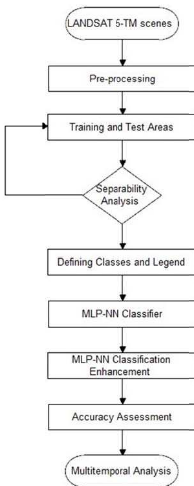
Fig. 3. Landsat data classification procedures
