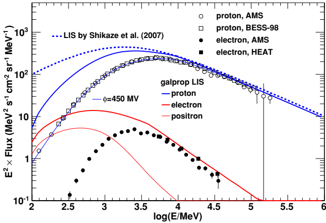
Figure 6. LIS of protons (thick blue line), and positrons (thin red line) used to calculate the \gamma -ray emissivity model in Figure 5 with a compilation of direct measurements at the Earth; see Alcaraz et al. (2000a), Sanuki et al. (2000), and Shikaze et al. (2007) for proton data and Alcaraz et al. (2000b) and Barwick et al. (1998) for electron data. Modulated spectrum with \phi = 450 MV is given by the thin blue line. The proton LIS adopted by Shikaze et al. (2007) is shown by the dotted blue line.
