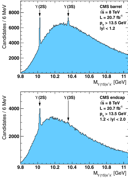
Fig. 1. The reconstructed invariant-mass distributions of the candidates in the barrel (top) and endcap (bottom) regions. Peaks corresponding to \Upsilon(2S) \rightarrow \Upsilon(1S)\pi^+\pi^- and \Upsilon(3S) \rightarrow \Upsilon(1S)\pi^+\pi^- decays are indicated with the arrows.
