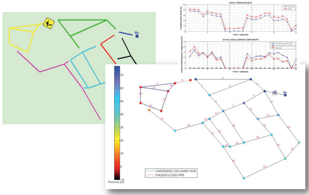
Fig. 2. WDNetXL can simulate the effects of WDN topology alterations in the same simulation time step.
