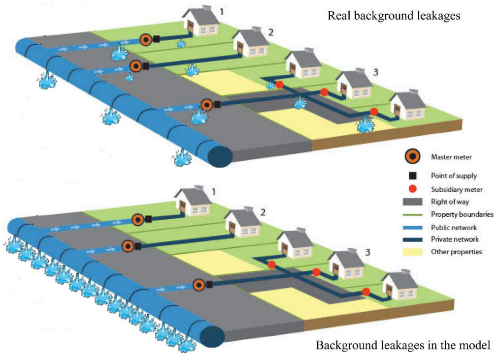
Fig. 3. Background leakages representation in WDNNetXL: the real background leakages in the WDN (upper figure) are represented as uniformly distributed background leakages along pipes in the WDN model, according to the Germanopoulos formulation.
