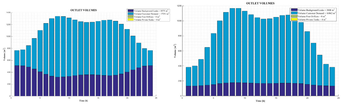
Fig. 7. Diagram of daily volumes of the different demand components before (left) and after (right) the installation of a PCV.
