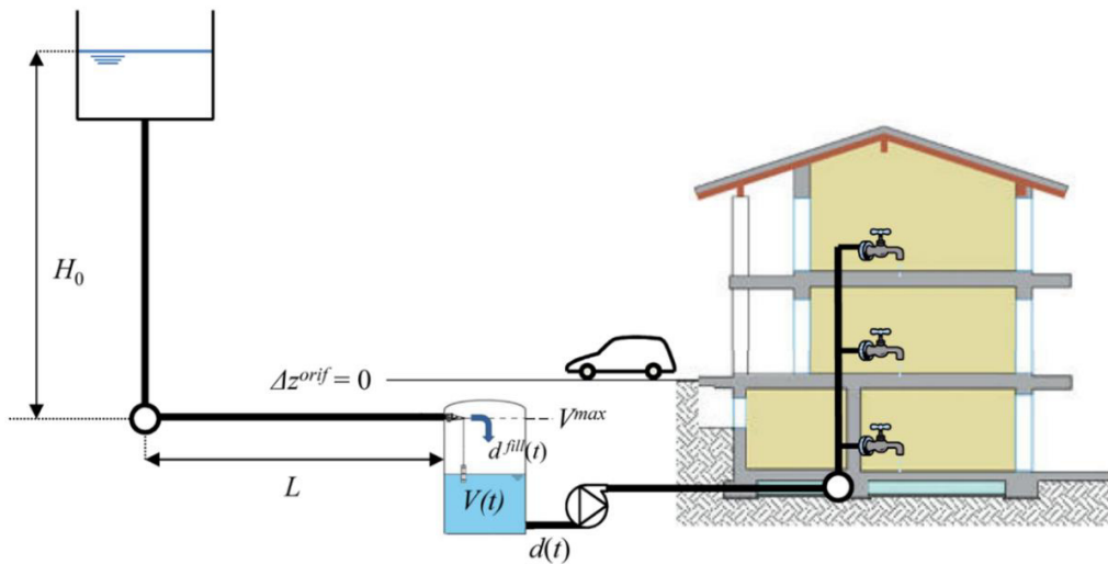
Fig. 4. Private local storage scheme assumed in the WDNNetXL hydraulic simulation.
