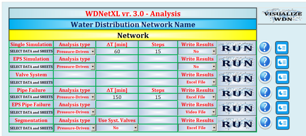
Fig. 1. User interface of WDNNetXL analysis module.
