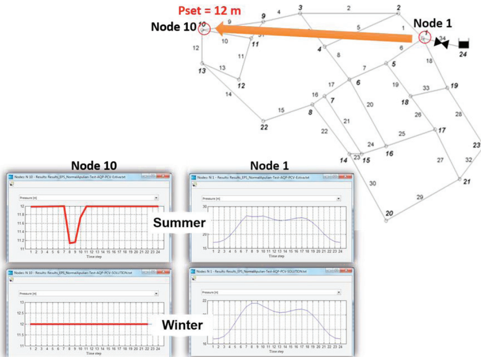
Fig. 6. Example of PCV (on pipe 34) controlled by pressure at node 10 at maximum (summer) and minimum (winter) demand scenarios. Note that when pressure at node 10 drops (at peak summer demand hour) the PCV is fully open, while in the winter scenario the PCV modulate pressure to actually match demand pattern.
