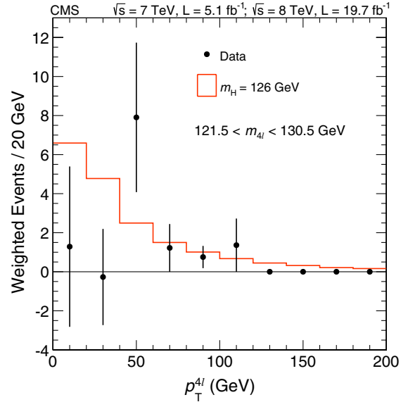
FIG. 15 (color online). s\mathcal{P} plot signal-weighted distribution of the four-lepton system p_T^{4\ell} for all the selected events in the mass region 121.5 < m_{4\ell} < 130.5 GeV. The red solid line represents the expectation from a SM Higgs boson.
