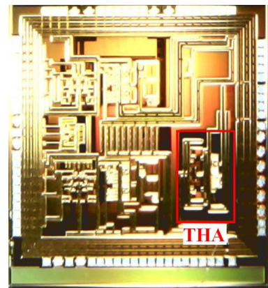
Fig. 8 Die photograph of the multi-function chip containing the prototype THA
