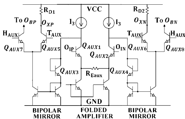
Fig. 7 Auxiliary amplifier
