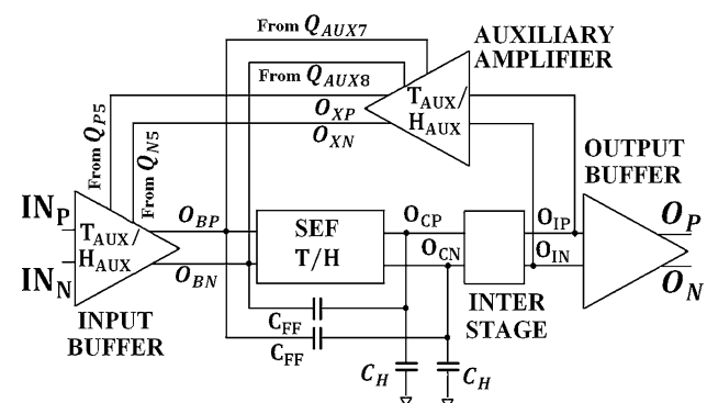
Fig. 1 THA architecture
