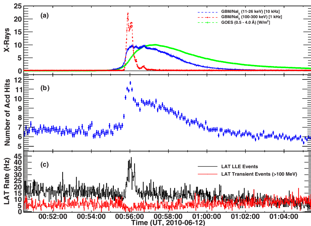
Figure 1. Time histories related to the 2010 June 12 solar flare. (a) GOES 0.5–4 Å rates, and GBM Na I 11–26 keV and 100–300 keV relative rates; (b) LAT ACD hit rate > 100 keV containing contributions from background, > 100 keV solar flare X-rays (impulsive peak) and pulse pile-up from tens of keV solar X-rays following the Na I 11–26 keV profile in (a); and (c) LLE and LAT Transient Class event rates.
