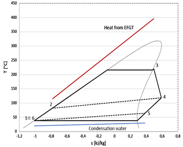
Fig. 2. Layout and T-s diagram ORC plant.
