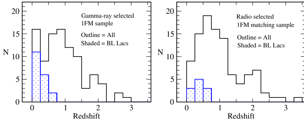
Figure 2. Left panel: redshift distribution of the \gamma -ray-selected IFM sample. The full sample is represented by the solid line, and the BL Lac objects are shaded. There is one radio galaxy (J0319+4130 = 3C 84) at z = 0.0176 . Right panel: redshift distribution for the radio-selected IFM matching sample. There are four radio galaxies in the sample, all in the first ( z < 0.25 ) bin.
