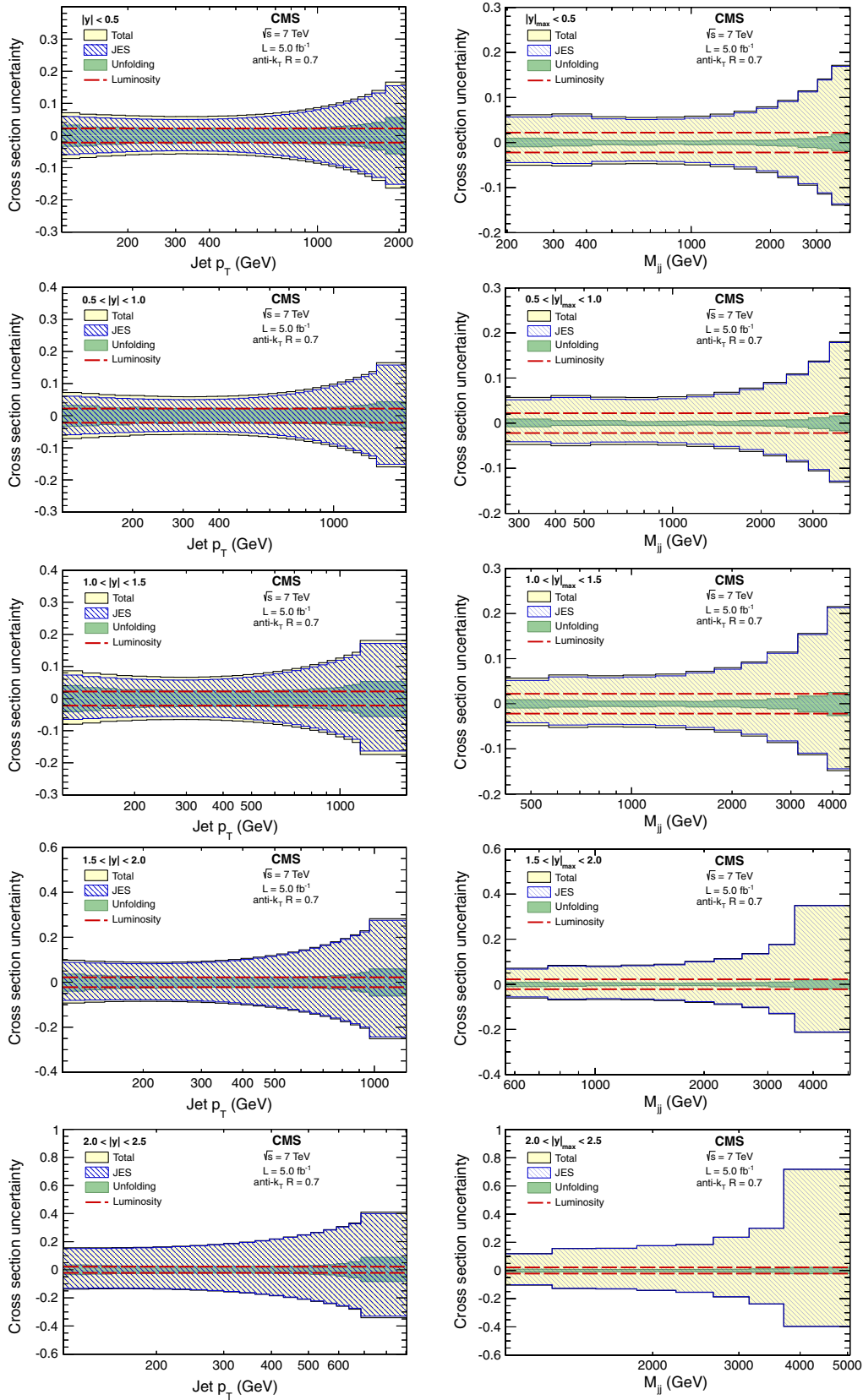
FIG. 5 (color online). Effect of the relative experimental uncertainties for the inclusive jet (left column) and dijet (right column) cross section measurements, and for all five |y| and |y|_{\text{max}} bins, respectively. The upward and downward uncertainties are estimated separately.
