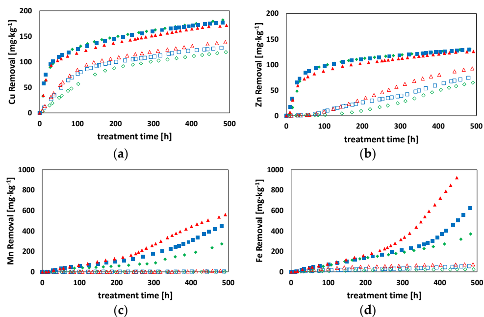
Figure 3. Breakthrough curves at different EBCTs with respect to treatment time. [EDDS] = 3.6 mM: \blacklozenge EBCT = 33 h; \blacksquare EBCT = 27 h; \blacktriangle EBCT = 21 h; [EDDS] = 0.36 mM: \diamond EBCT = 33 h; \square EBCT = 27 h; \triangle EBCT = 21 h—(a) Cu; (b) Zn; (c) Mn; (d) Fe.
