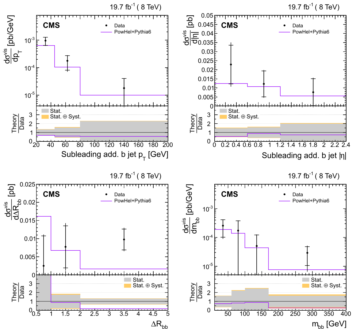
Fig. 16 Absolute differential t\bar{t} cross section measured in the visible phase space of the t\bar{t} system and the additional b jets, as a function of the second additional b jet p_T ( top left ) and |\eta| ( top right ), the angular separation \Delta R_{bb} between the two leading additional b jets ( bottom left ),
