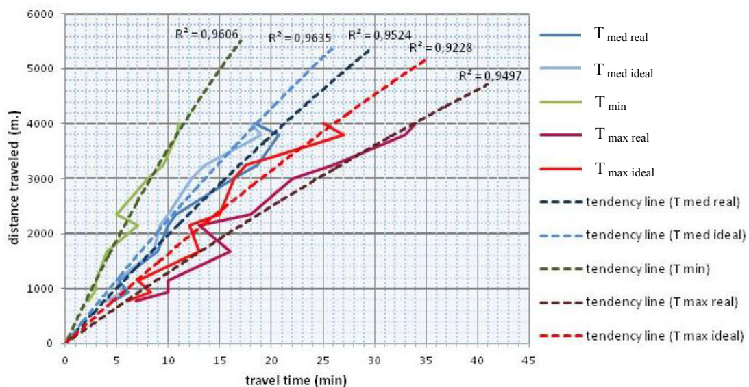
Fig. 3 – bicycle space/time graph
