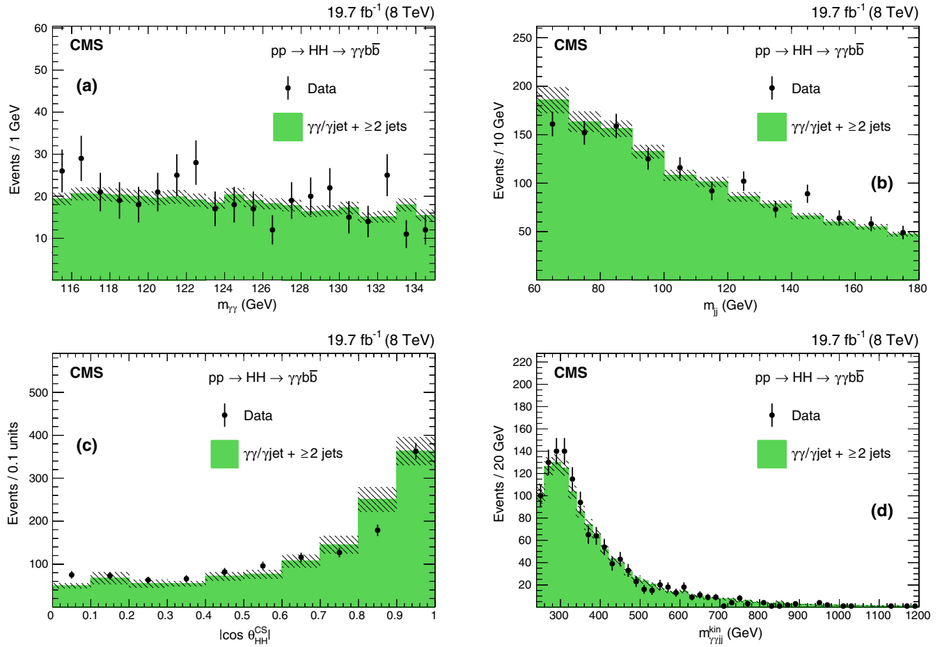
FIG. 1. Reconstructed spectra for data compared to the \gamma\gamma/\gamma\text{jet} + \geq 2\text{jets} background after the selections described in Table I (selections on photons and jets and a requirement of at least one b -tagged jet): (a) m_{\gamma\gamma} , (b) m_{jj} , (c) |\cos\theta_{HH}^{\text{CS}}| , and (d) m_{\gamma\gamma jj}^{\text{kin}} . The hatched area corresponds to the bin-by-bin statistical uncertainties on the background prediction reflecting the limited size of the generated MC sample. The comparison is provided for illustrative purpose, the backgrounds, except the one coming from single-Higgs-boson production, are evaluated from a fit to the data without reference to the MC simulation.
