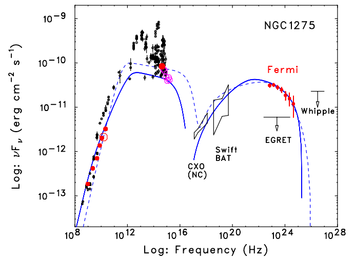
Figure 7. Overall SED of NGC 1275 constructed with multiband data, using radio (RATAN-600 in filled red circle; this work), radio core (MOJAVE in open red circle; this work), optical (MITSuME in red; this work), optical/UV ( Swift /UVOT in open magenta circle; this work), radio to X-ray (NED), nonthermal X-ray nuclear emission (Balmaverde et al. 2006), hard X-ray ( Swift /BAT; reconstructed from Ajello et al. 2009), EGRET upper limit (Reimer et al. 2003), Whipple upper limit (Perkins et al. 2006), and Fermi (this work). The RATAN, MOVAVE and MITSuME data are contemporaneous with the Fermi data. Swift UVOT data come from most recent archival observation in December 2007. The SED is fitted with a one-zone synchrotron/SSC model (blue dashed curve) and a decelerating flow model (Georganopoulos & Kazanas 2003b; blue solid curves). See the text for parameters.
