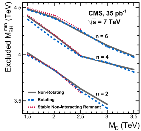
Fig. 4. The 95% confidence level limits on the black hole mass as a function of the multidimensional Planck scale M_D for several benchmark scenarios. The area below each curve is excluded by this search.
