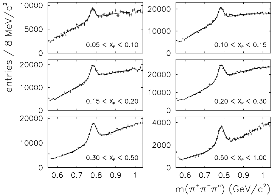
Fig. 2. Fits in the \omega region made to the invariant mass spectra of data (like-sign subtracted).
