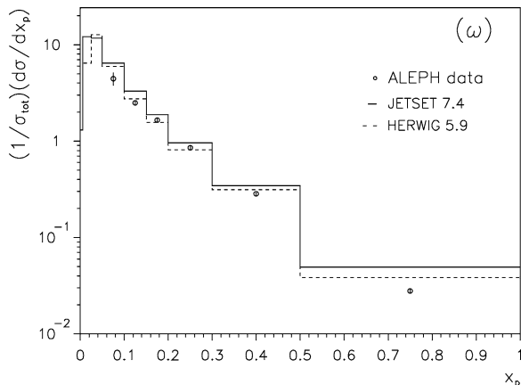
Fig. 4. Measured differential cross sections for the \omega in comparison with Monte Carlo predictions. The errors shown are the quadratic sum of statistical and systematic contributions.
