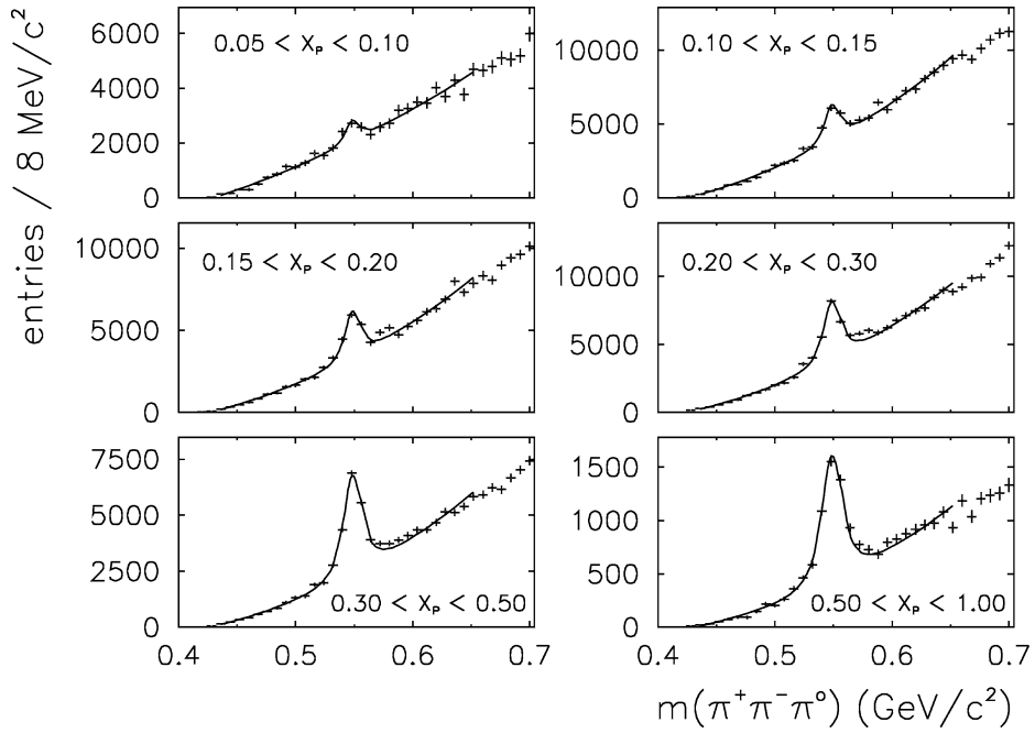
Fig. 1. Fits in the \eta region made to the invariant mass spectra of data (like-sign subtracted).
