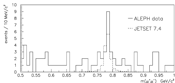
Fig. 6. Invariant mass distribution m(\mu^+\mu^-) for hadronic events containing a muon pair with tighter cuts (as explained in the text). The \omega signal of JETSET is normalized to the signal in the data shown.
