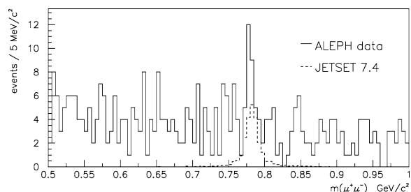
Fig. 5. Invariant mass distribution m(\mu^+\mu^-) for hadronic events containing a muon pair after standard cuts as described in the text. The \omega signal of JETSET is normalized to the signal in the data shown.
