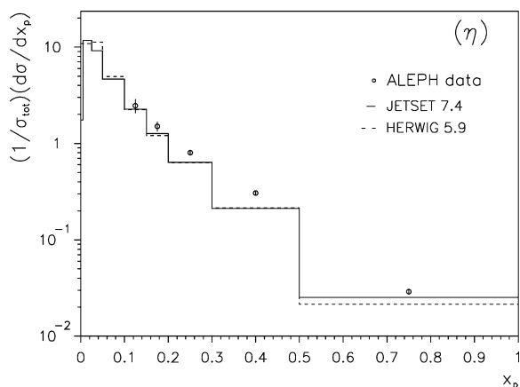
Fig. 3. Measured differential cross sections for the \eta in comparison with Monte Carlo predictions. The errors shown are the quadratic sum of statistical and systematic contributions.
