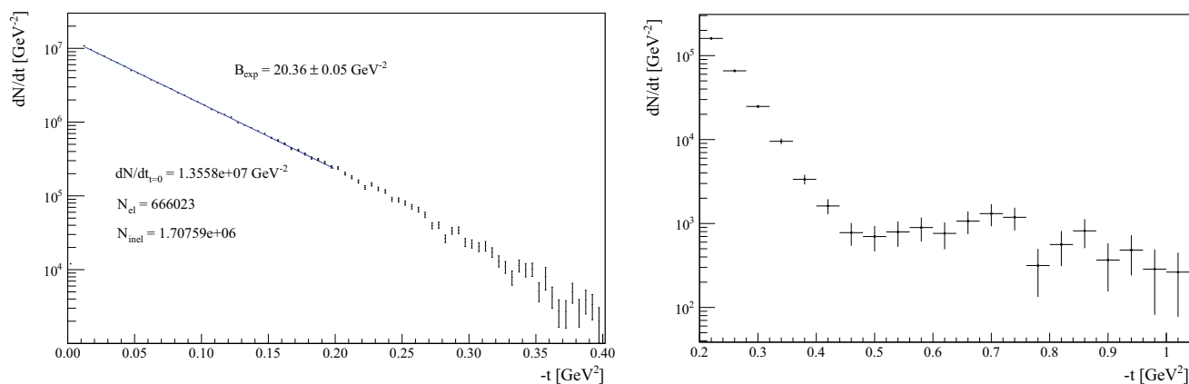
Fig. 3 Differential elastic rate dN_{\text{el}}/dt at \sqrt{s} = 13 TeV (full physics corrections included) of dataset DS2 with the exponential fit between |t|_{\text{min}} and |t|_{\text{max}} . The right panel shows the data in the dip region. The uncertainties shown and quoted are only statistical
