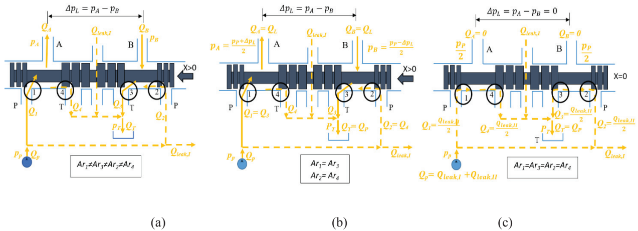
FIGURE 1. Schematization of a spool inside a bushing sleeve: generic valve with a spool displacement x (a), symmetrical valve with a spool displacement x (b), symmetrical valve with the spool at null and zero pressure load across the actuator (c)
