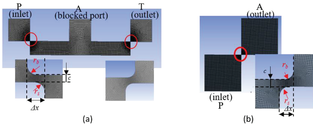
FIGURE 3. 2D computational grids for an existing valve showing the case with radius r_b = r_s = 4 \mu\text{m} , clearance c = 3 \mu\text{m} and overlap \Delta x_{P-A} = 7 \mu\text{m} and \Delta x_{A-T} = 5 \mu\text{m} (a), and simplified domain showing the case with radius r_b = r_s = 4 \mu\text{m} , clearance c = 3 \mu\text{m} and overlap \Delta x = 6 \mu\text{m} (b)
