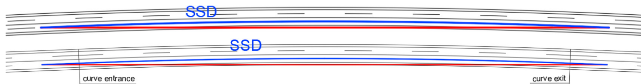
Fig. 4. (top) limiting stopping sight distance included in the curve length; (bottom) limiting stopping sight distance greater than the curve length.
