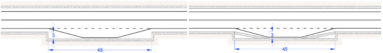
Fig. 3. (left) local widening of the tunnel cross-section in correspondence with lay-bys (with example measures taken from Italian standards). (right) solution representing the implementation of oblique vertical walls in presence of lay-bys.
