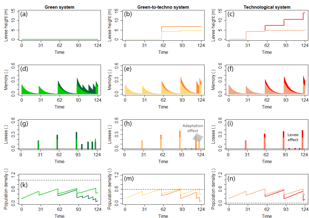
Figure 12. Levee height ( H ), collective memory ( M ), flood losses ( FD ), and population density ( D ) dynamics of green (a, d, g, k), green-to-techno (b, e, h, m), and technological (c, f, i, n) systems. The lighter colour indicates scenario 1 and the darker colour indicate scenario 4. Dashed lines indicate the values of the \delta_D parameter.
