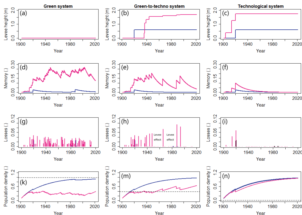
Figure 5. Levee height ( H ), collective memory ( M ), flood losses ( FD ), and population density ( D ) dynamics of green (a, d, g, k), green-to-techno (b, e, h, m), and technological (c, f, i, n) systems for values of the level of bias \beta equal to 1 (blue) and 10 (magenta). Dashed lines indicate the values of the \delta_D parameter.
