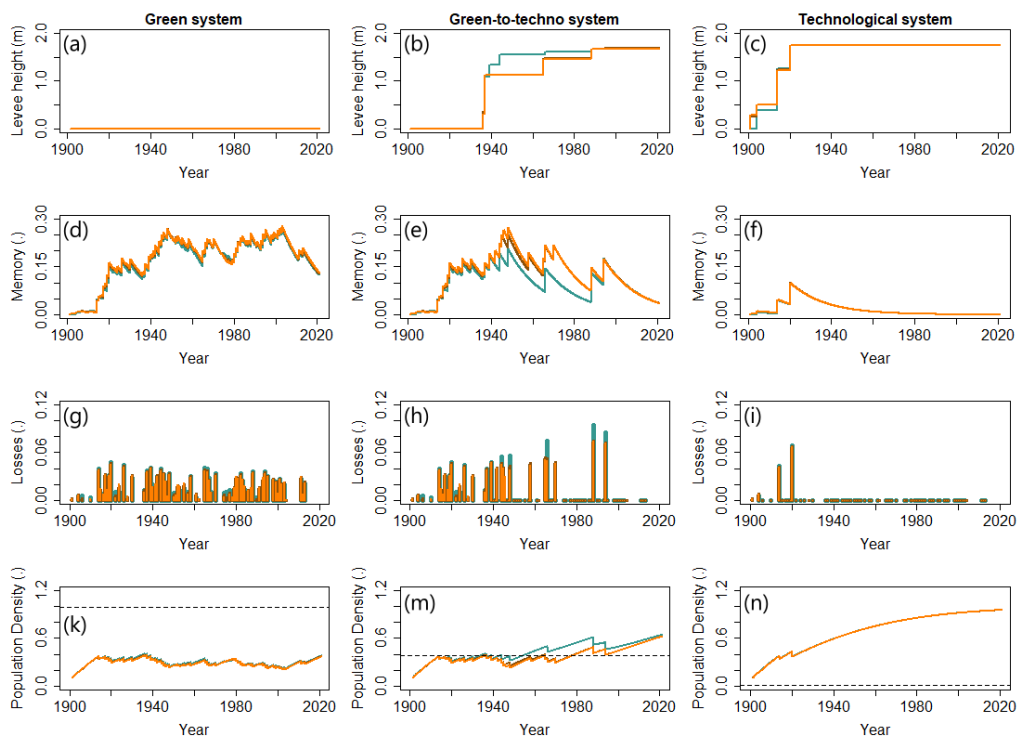
Figure 7. Levee height ( H ), collective memory ( M ), flood losses ( FD ), and population density ( D ) dynamics of green (a, d, g, k), green-to-techno (b, e, h, m), and technological (c, f, i, n) systems for values of memory decay rate \mu equal to 0.10 \text{ year}^{-1} (light green), 0.15 \text{ year}^{-1} (brown), and 0.20 \text{ year}^{-1} (orange). Dashed lines indicate the values of the \delta_D parameter.
