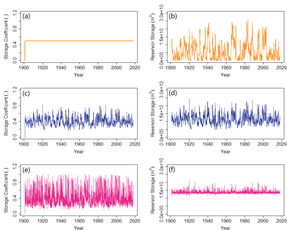
Figure 3. Variation of the storage coefficient (a, c, e) and the reservoir storage (b, d, f) for three different values of the level of bias \beta equal to 0 (orange), 1 (blue), and 10 (magenta).
