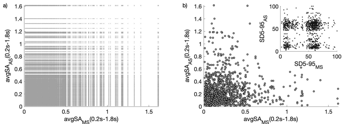
FIGURE 4 Scatter of avgSA for mainshock (MS) versus aftershock (AS). (a) All possible pairs (391,876 sequences); (b) randomly selected 1000 sequences via the Latin hypercube sampling approach. SD5-95:
