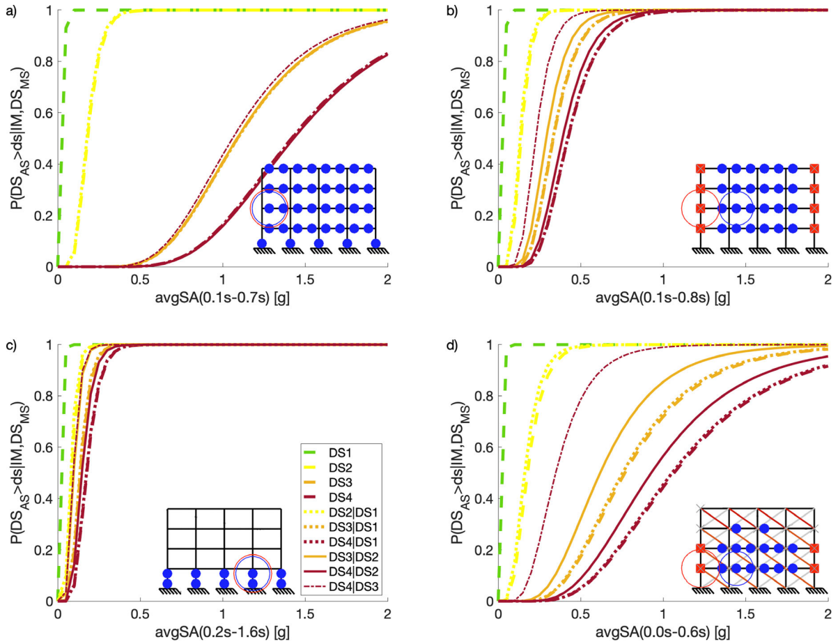
FIGURE 9 State-dependent fragility (four-storey frames). (a) Beam sway; (b) mixed sway; (c) column sway; (d) mixed sway infilled. Note: The line type represents the conditioning damage state ( DS_{MS} ) while the line color represents the achieved damage state ( DS_{AS} ). For example, the red dotted line represents DS_{MS} = 1 and DS_{AS} = 4
