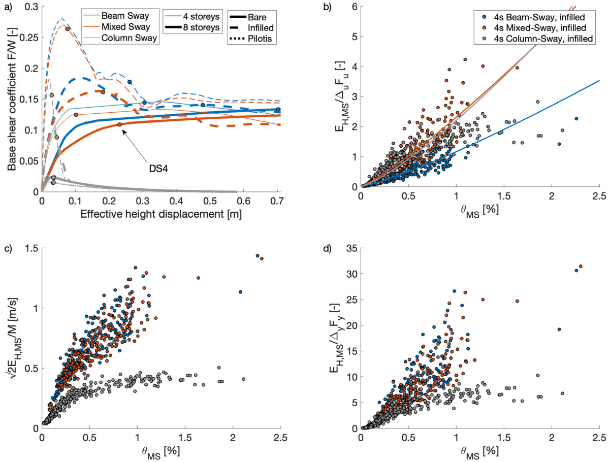
FIGURE 8 (a) Normalized pushover curves. F : base shear, W : total weight; (b) normalized hysteretic energy versus maximum interstorey drift for the four-storey infilled case studies. \Delta_y, F_y : displacement and base shear at yielding (DS2); \Delta_u, F_u : displacement and base shear at damage state 4; M : total mass
