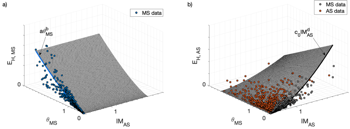
FIGURE 5 Derivation of the probabilistic seismic demand model. (a) Mainshock; (b) aftershock
